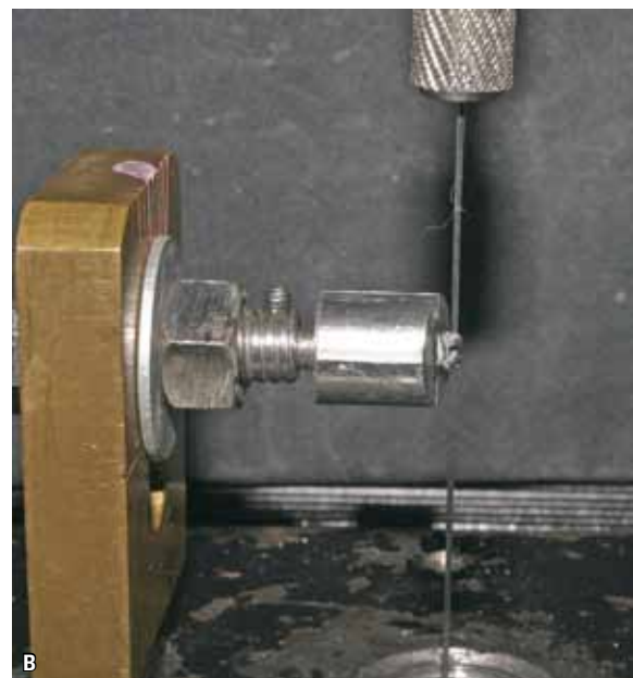
FIGURE 2 - A) Front view of self-ligating bracket bonded to metal cylinder with compensatory angulation to ensure traction is performed with no pre-angulation or torque. Total absence of angulation (tip) can be confirmed by the vertical alignment of the markings on the metal cylinder and copper colored part seen in the background. B) Side view of the same bracket described during traction of stainless steel 0.019 x 0.025-in cross-section wire.
