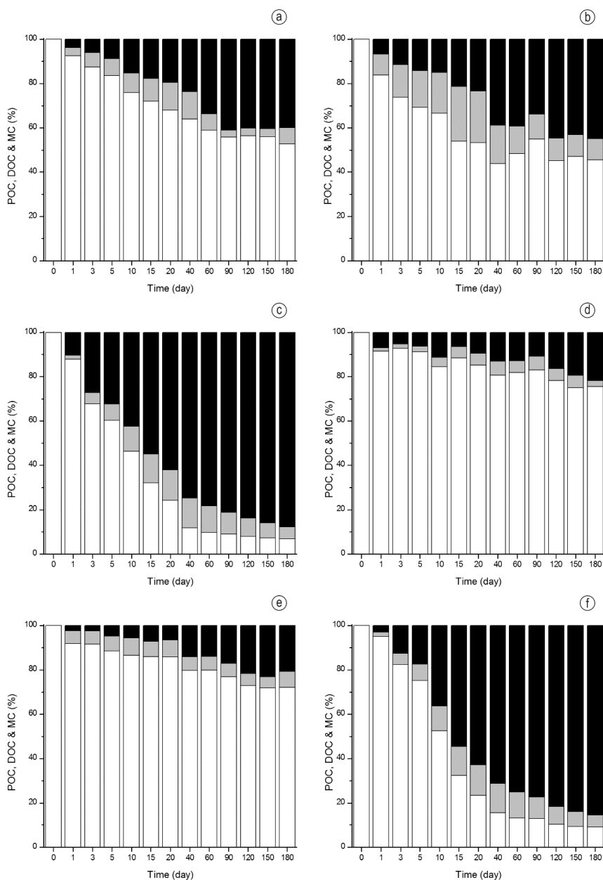
Figure 2. Carbon budget from the anaerobic mineralization of Salvinia auriculata (a = integral detritus; b = POC and c = DOC) and Utricularia breviscapa (d = integral detritus; e = POC and f = DOC). Where: particulate organic carbon (POC) = white bar; dissolved organic carbon (DOC) = gray bar and mineralized carbon (MC) = black.
