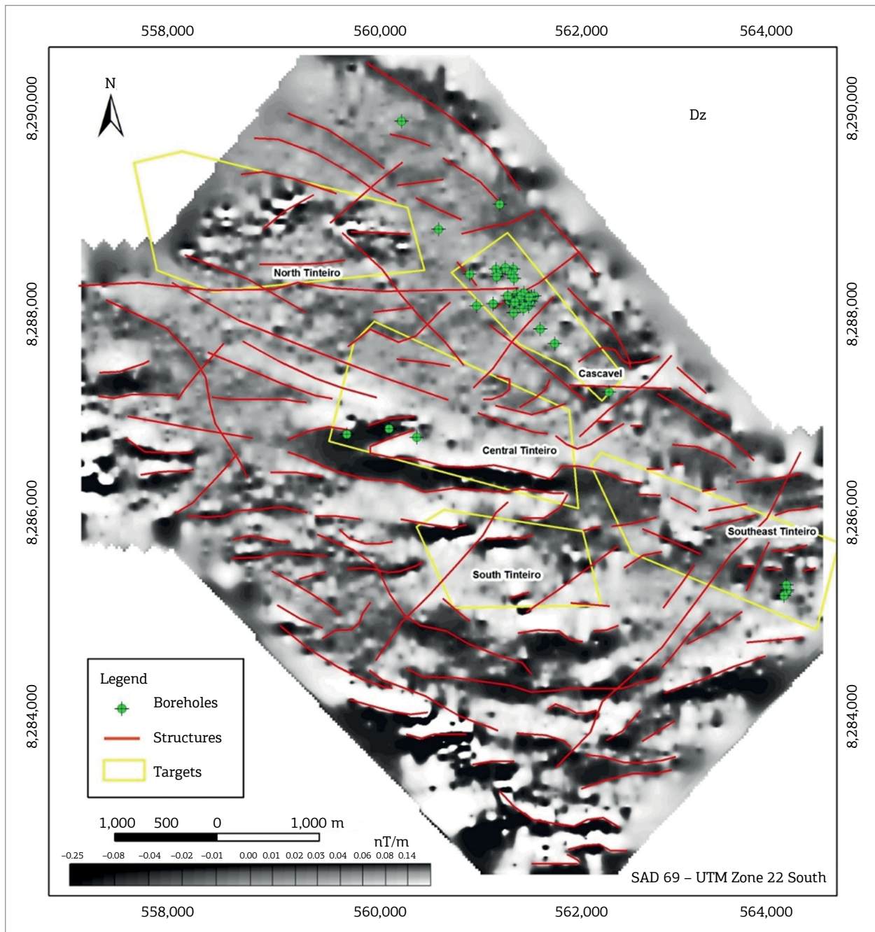
Figure 7. Map showing the first vertical derivative ( Dz ) of the TMI in the study area and identifying the main geologic structures interpreted based on the Dz , Dy , and RGB 453 image of the Landsat 7 ETM+ sensor. The boreholes conducted by the Orinoco do Brasil Mineração Ltda. are indicated by the green marker.
