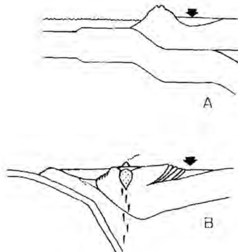
Fig. 5. Contrasting theories on the formation of a foreland basin. A. Foreland basin caused by a shallowly subducted plate (redrawn from Cross and Pilger, 1982). B. Foreland basin caused by isostatic adjustment to a backarc fold-thrust belt (redrawn from Dickinson, 1976). Arrows indicate subsidence in the foreland basin.
