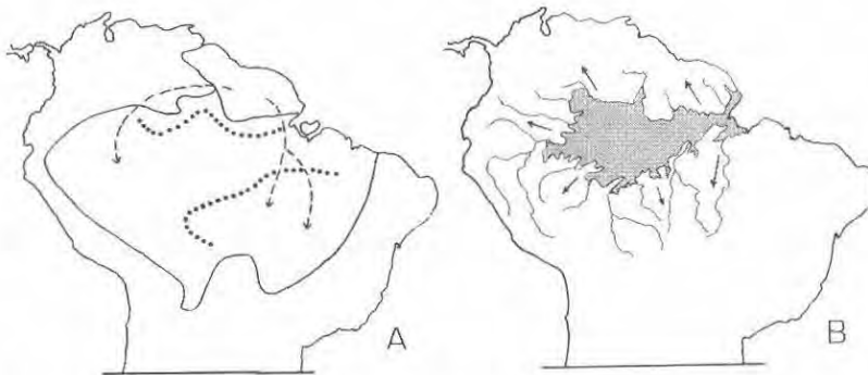
Fig. 9. A. Hypothesized paths of range extensions in some Amazonian fishes (from Géry, 1964). B. A reduced Lago Amazonas, drawn on the 100 m contour line, with hypothesized relictual distribution of lake fish in the newly formed river channels.
