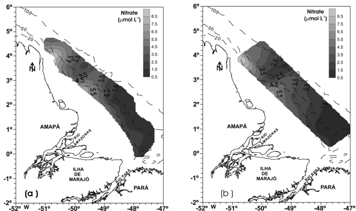
Fig. 8 – Distribution of the superficial concentration of the nitrate during Operation Norte IV (falling discharge of the Amazon river): (a) REVIZEE data; and (b) MACC-2D model results.
