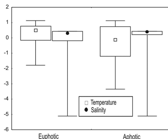
Fig. 3 – Autoscaled value distributions for temperature and salinity.
