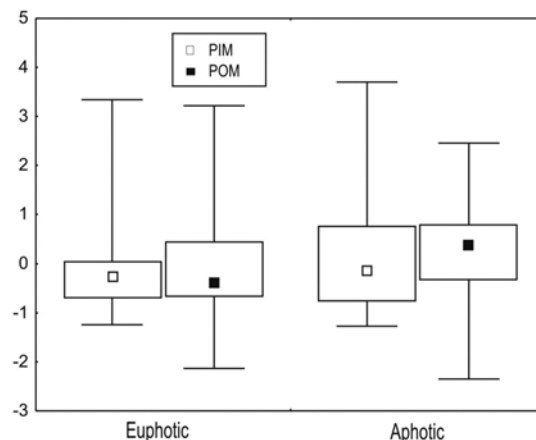
Fig. 5 – Autoscaled value distributions values for suspended particulate inorganic (PIM) and organic (POM) materials.
