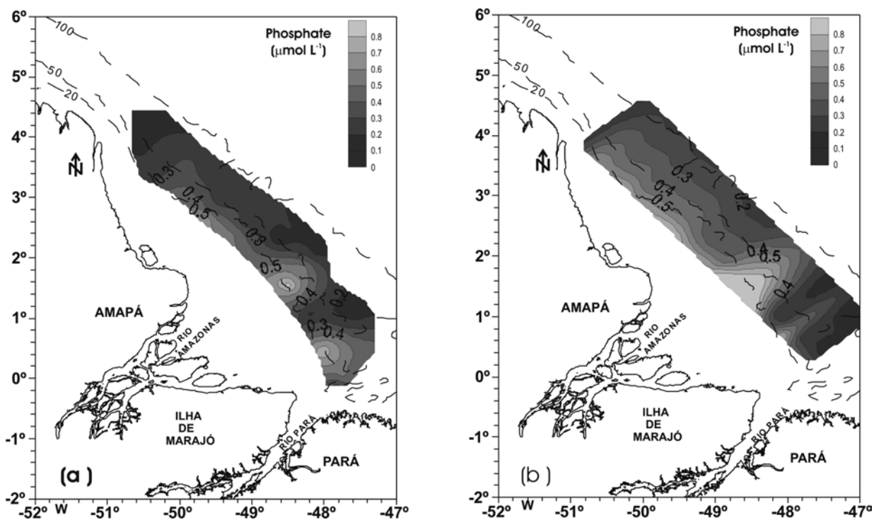
Fig. 9 – Distribution of the superficial concentration of the phosphate during Operation Norte III (high discharge of the Amazon river): (a) REVIZEE data; and (b) MACC-2D model results.
