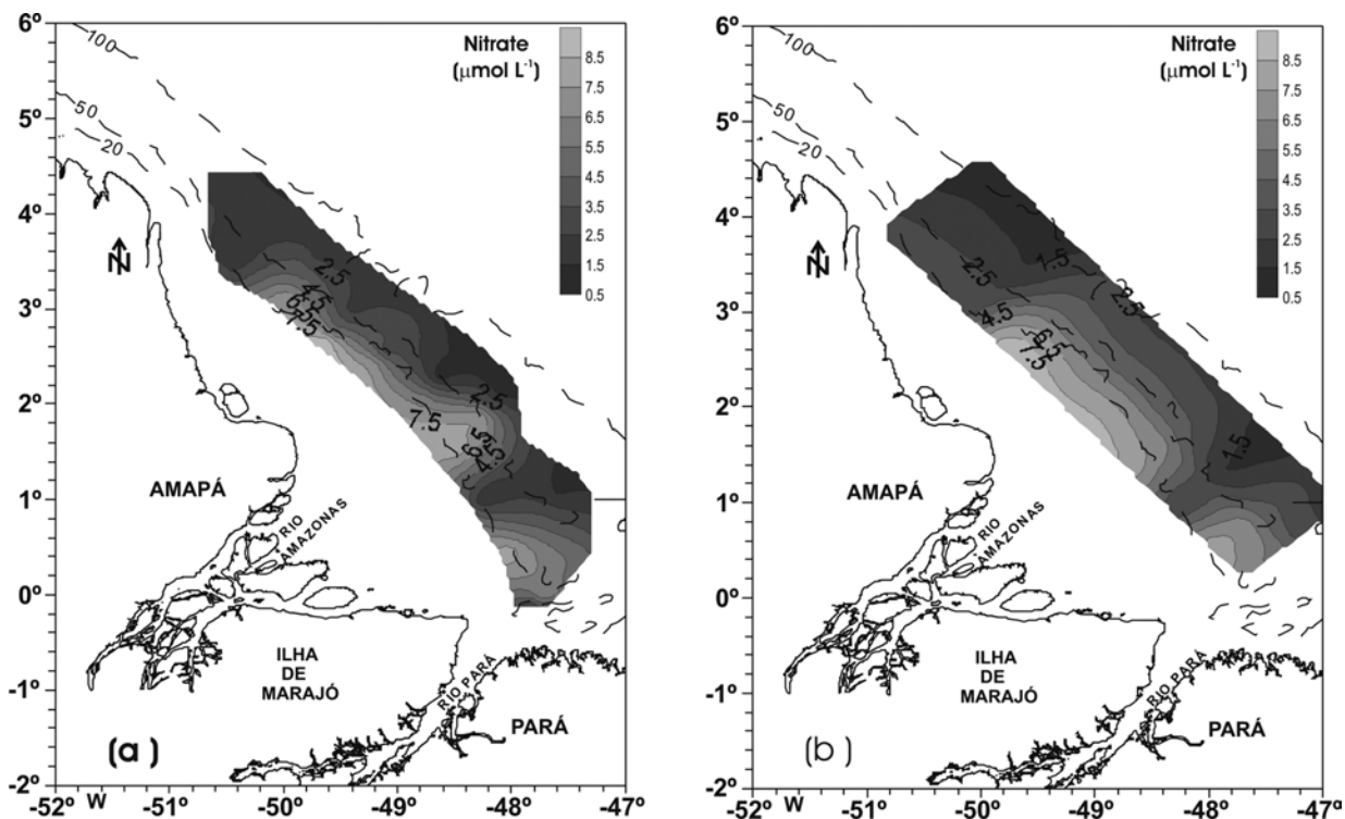
Fig. 10 – Distribution of the superficial concentration of the nitrate during Operation Norte III (high discharge of the Amazon river): (a) REVIZEE data; and (b) MACC-2D model results.
