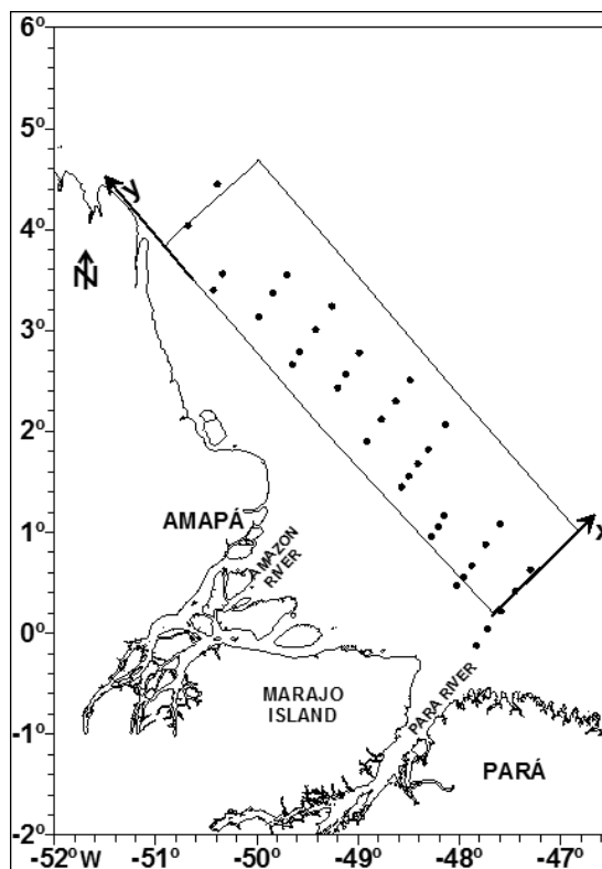
Fig. 2 – Map of the stations of the REVIZEE Program, and the integration domain used in the simulations with MAAC-2D.
