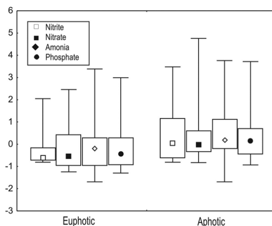
Fig. 4 – Autoscaled value distributions for nitrite, nitrate, ammonia and phosphate.
