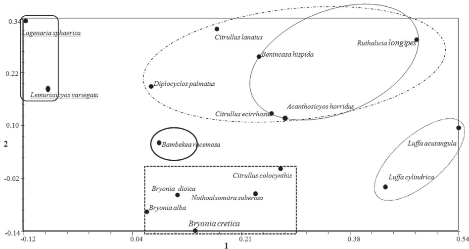
Figure 6. Scatterplot of the 16 OTUs plotted against the first principal coordinate by the second principal coordinate.
