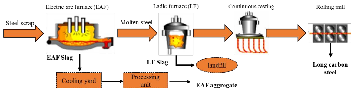
Figure 1 - Schematics of the steelmaking process, depicting the generation of EAFS and its management
