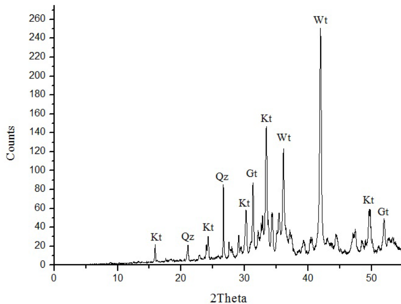
Figure 2 - XRD pattern of EAF aggregate used in concrete paving blocks
