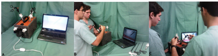
FIGURE 7 – Finished model. A. New experimental model. B. Use and image obtained in the laptop screen simultaneously C. Model in use.
