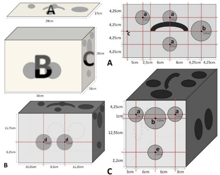
FIGURE 1 – Project for the construction of the experimental model. A. Housing cover project B. Lateral wall project C. Front wall project. a. Hole (45 mm) for introduction of trocars. b. Hole (65 mm) for camera input. c. Hole for security lock d. Hole (65 mm) for common and videosurgical instruments. e. Hole (45 mm) for attaching the nozzle to the lamp.
