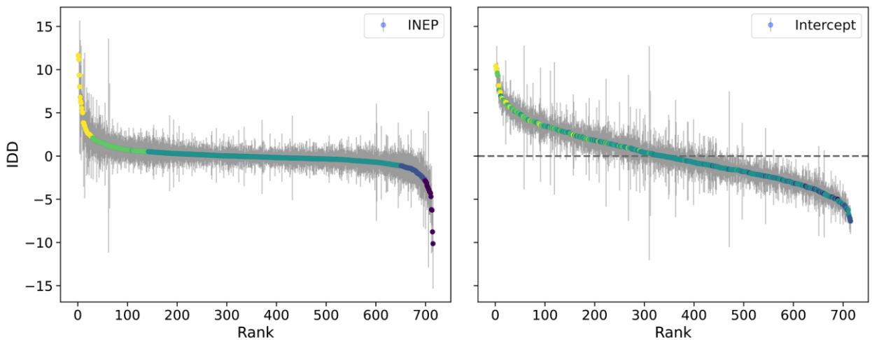
Figure 4 - Same data as in Fig. 3, but with courses ordered by rank and an estimate of the standard error
