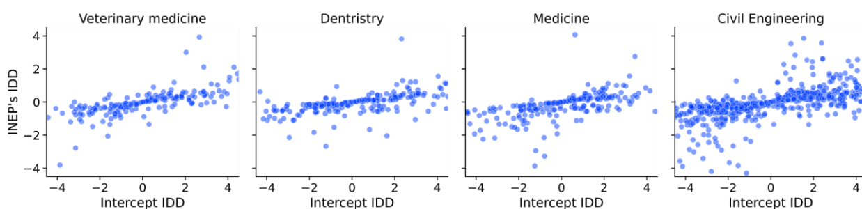
Figure 2 - Comparison between INEP and Intercept IDD values
