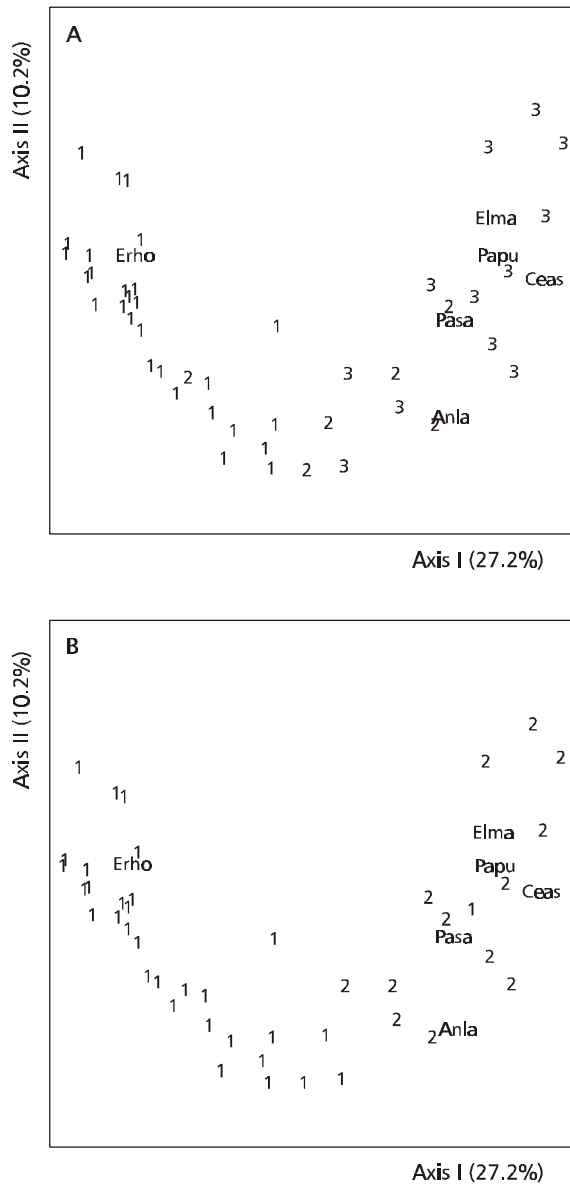
Fig. 1 – Ordination of 46 grassland communities (quadrats 1.5 x 0.5 m) in Eldorado do Sul, RS, Brazil. The scatter diagram is defined by ordination axes 1 and 2 generated by principal coordinates analysis from chord distances using the species composition data. The percentage of total variation represented by the axes is indicated. The species plotted on the diagram had a correlation |r| \geq 0.6 with at least one of the axes: Erho = E. horridum ; Anla = A. lateralis ; Pasa = P. sabulorum ; Ceas = C. asiatica ; Papu = P. pumilum ; and Elma = E. maculosa . Diagrams A and B are identical except that in A the numbers 1-3 identify the soil moisture state of the quadrat (scale in the main text) and in B the numbers 1-2 identify the community types revealed by cluster analysis.
