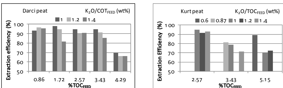
Figure 4: Peat extraction efficiency (total organic carbon extracted per unit total organic carbon in the peat) for varying amounts of peat (expressed as TOC FEED ) and alkali additions (expressed as the K 2 O/TOC FEED ). Darci (left) and Kurt peat (right).
