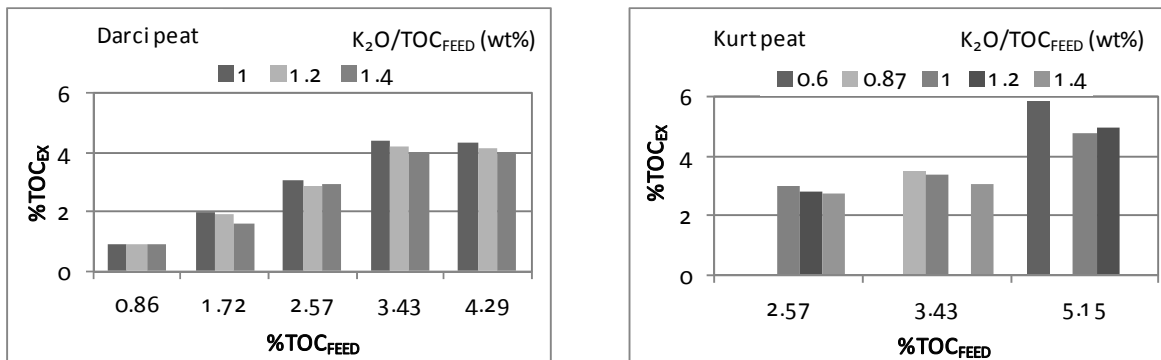
Figure 3: Total organic content in the extraction mixture (TOC EX ) for varying amounts of peat (expressed as TOC FEED ) and alkali additions (expressed as the K 2 O/TOC FEED ). Darci (left) and Kurt peat (right). The extraction lasted 24 h.
