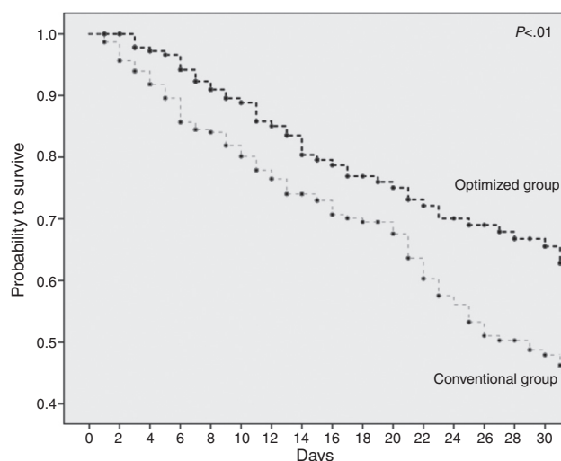
Fig. 1 – Survival curves of different ASP strategies.
