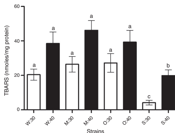
Fig. 3 – Lipid peroxidation in yeast strains (W: W303-1A, M: MC4, O: OFF1, and S: SLP1) under normal temperature condition 30 (30 °C) and increased temperature 40 (40 °C for 2 h). Other conditions are as described in ‘Materials and methods’ section. Each value represents the mean \pm SEM (Standard Error of the Mean) ( n=3 ). Significant differences ( ^b p < 0.05 and ^c p < 0.01 ), with respect to W303-1A.
