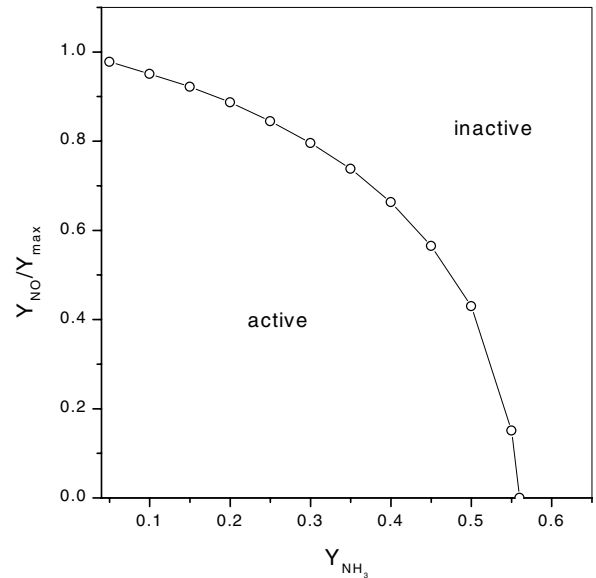
Figure 3. Phase diagram in the plane normalized adsorption rate of nitrogen monoxide versus Y_{NH_3} . The points indicate the phase transition between the active and inactive phases. The line is a guide to eyes.
