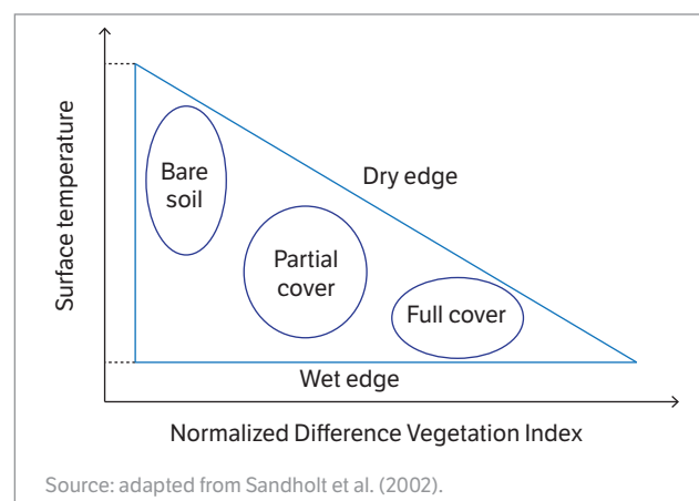
Figure 3. Evaporative triangle.
