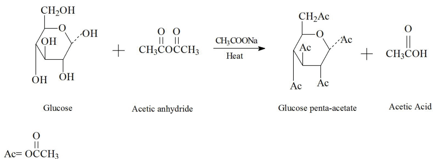
Figure 2: Scheme for the synthesis of acylsugar 2 (glucose penta-acetate).
