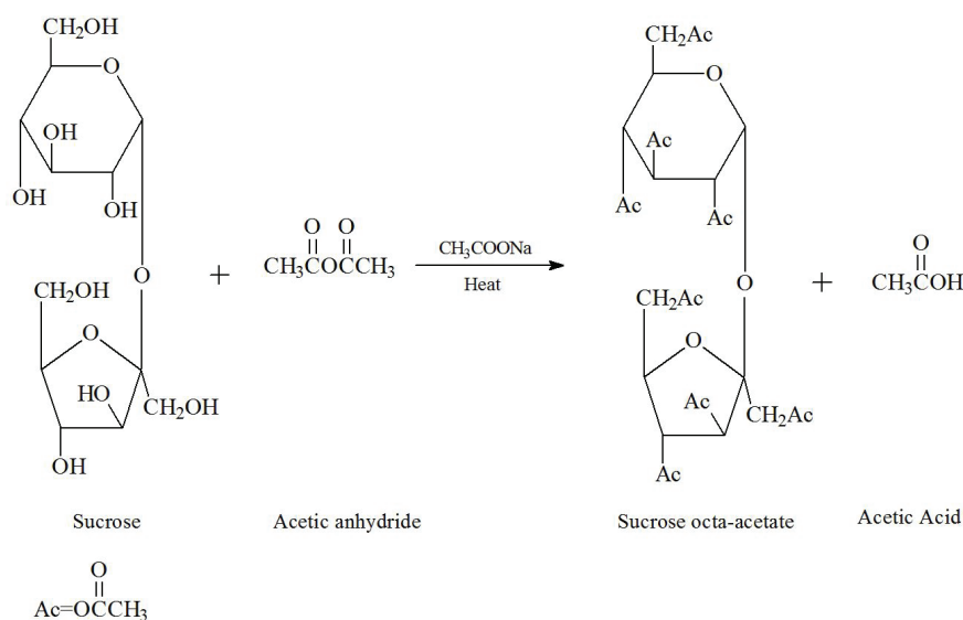
Figure 1: Scheme for the synthesis of acylsugar 1 (sucrose octa-acetate).
