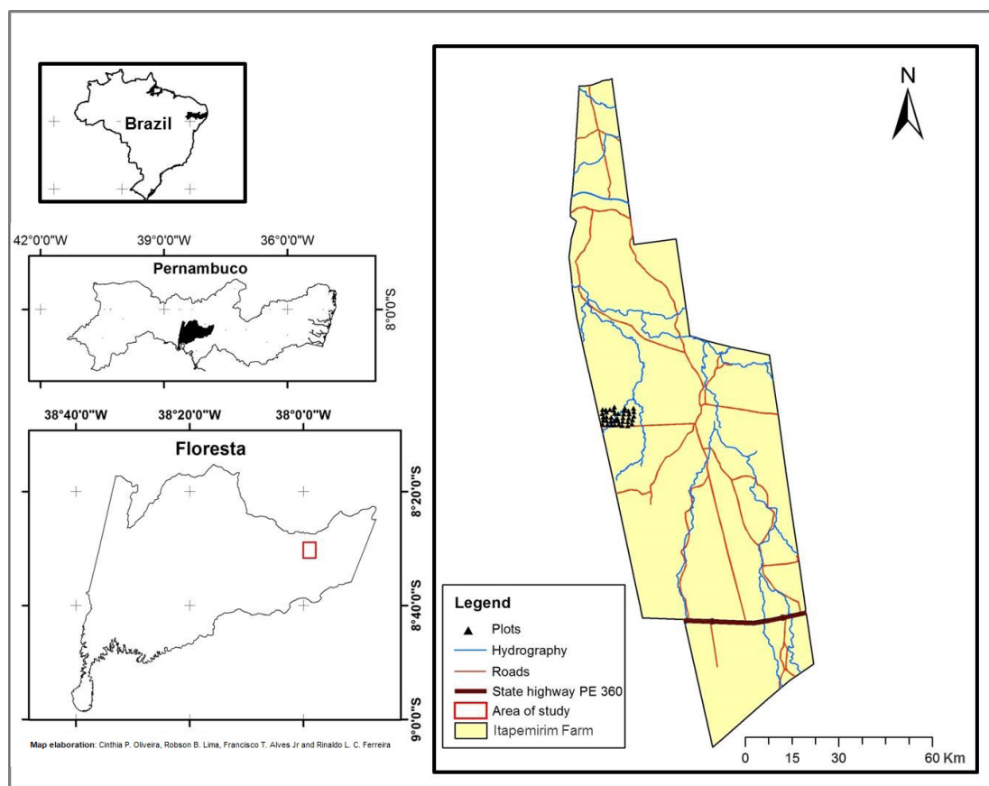
Figure 1. Location of the study area in the municipality of Floresta, state of Pernambuco, Brazil. Source: Lima et al. (2017).
