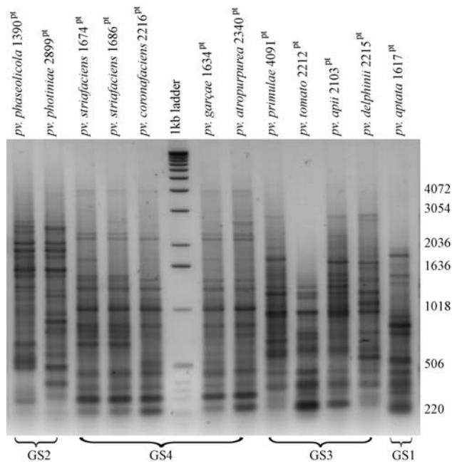
Figure 4 - Agarose gel electrophoresis of BOX-PCR fingerprinting patterns from genomic DNA of different pathovars belonging to Pseudomonas syringae (pathovars photiniae , striafaciens , coronafaciens , garçae , atropurpurea , primulae , tomato , apii , delphinii and aptata ) and P. savastanoi pv. phaseolicola , which represent some of the nine known genomic species (GS), assigned after Gardan et al. (1999). Isolates obtained from the “Collection Française des Bactéries Phytopathogènes” (CFBP, Angers, France). The molecular size marker is a 1-kb ladder (Gibco BRL Life Technologies Inc.) and the sizes are indicated in base pairs. Shown is a negative image of an ethidium bromide gel. pt : pathotype strain.
