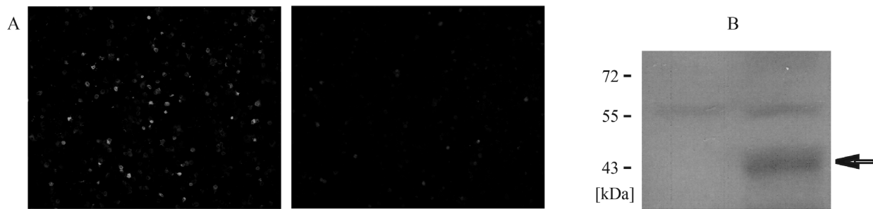
Figure 3 - Expression of a CD9-C-EGFP fusion protein in BT4Ca cells. To confirm that from the ATG located in the extension of exon 2 of CD9 mRNA-C a protein can be translated, the variant CD9 sequence was inserted in a vector to express a fusion protein with C-terminal EGFP only if a functional start codon was provided. For all constructs, three parallel transfections were performed leading to undistinguishable results. (A) Bright fluorescence indicated expression of a fusion protein after transfection of BT4Ca cells (left). In a control transfection, a construct in which the CD9 stop codon had not been removed was used (right). (B) Lysates from transfectant cells were analysed by Western blot with an anti-EGFP antibody recognizing the fusion protein (right lane) which was not detected in cells transfected with the control plasmid (left lane).
