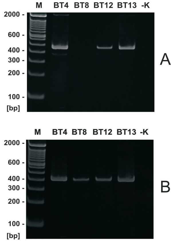
Figure S1 - RT-PCR analyses of CD9 expression by rat BT cell lines. cDNAs were prepared from RNAs expressed by different rat BT cell lines and used as templates in subsequent PCRs with primer pairs covering the first exons (A) or the last exons (B) of the CD9 gene. Lack of a specific PCR product suggested that BT8Ca cells predominantly express a CD9 transcript with a different 5'-end.
