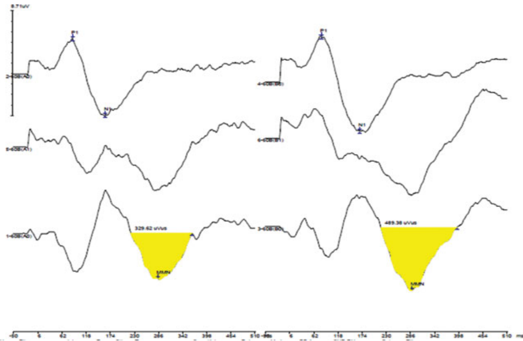
Fig. 1 MMN plot for the contrasts of [da] (frequent) and [ta] (rare) and the resulting (frequent) stimuli of a sample subject.
