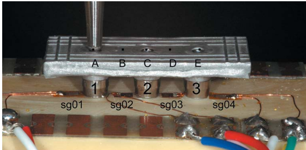
Figure 2- Detail of static vertical loading on loading point A
