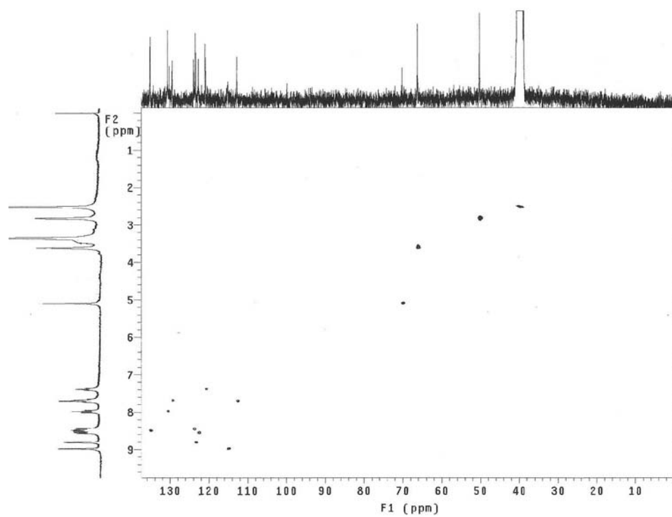
Figure S54. HMQC spectra of compound 7b.
