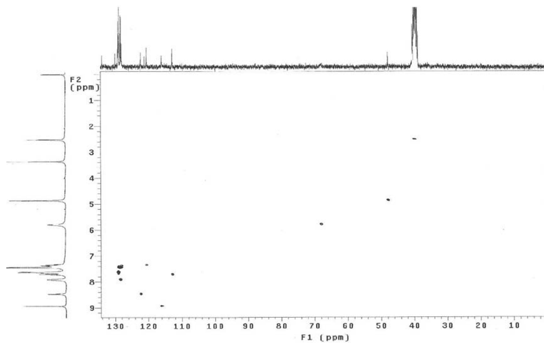
Figure S34. HMQC spectra of compound 5a .
