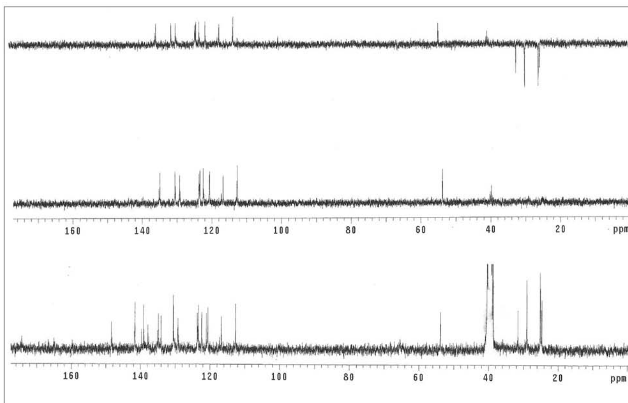
Figure S27. ^{13}\text{C} NMR / DEPT spectra (75.5 MHz, \text{DMSO-}d_6 ) of compound 4b .
