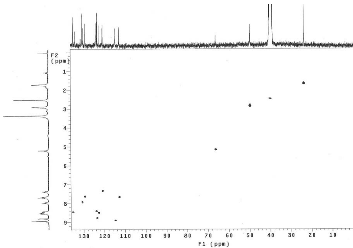
Figure S46. HMQC spectra of compound 6b .
