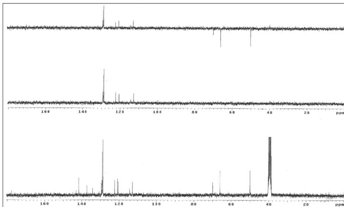
Figure S50. ^{13}\text{C} NMR / DEPT spectra (75.5 MHz, \text{DMSO}-d_6 ) of compound 7a.
