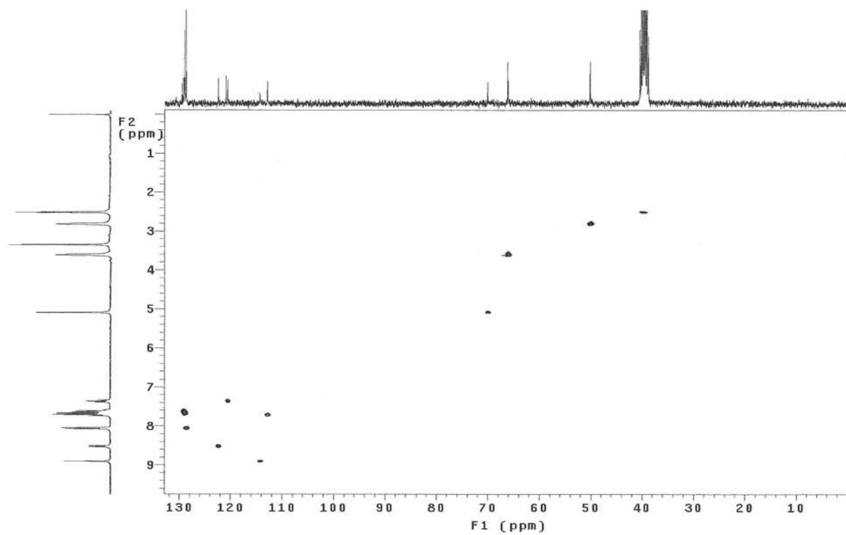
Figure S51. HMQC spectra of compound 7a.
