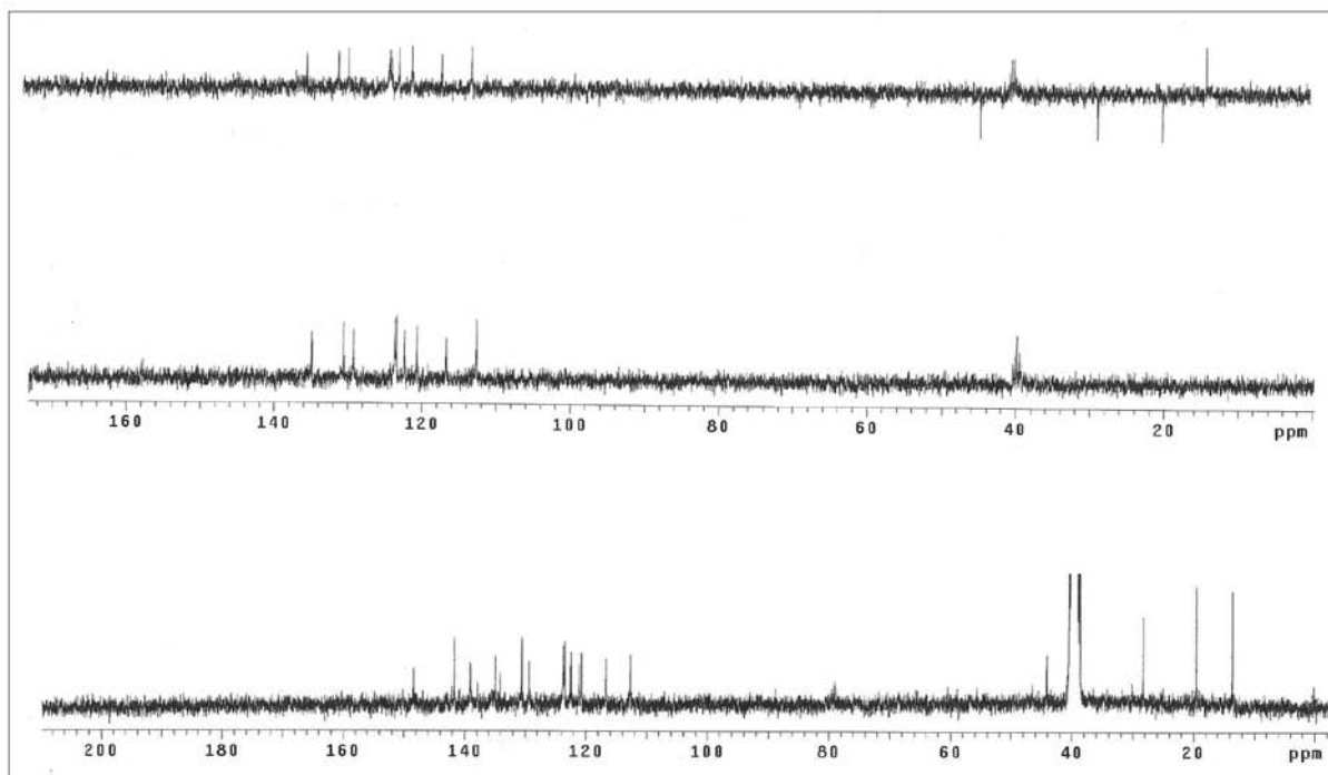
Figure S18. ^{13}\text{C} NMR / DEPT spectra (75.5 MHz, \text{DMSO-}d_6 ) of compound 3b .
