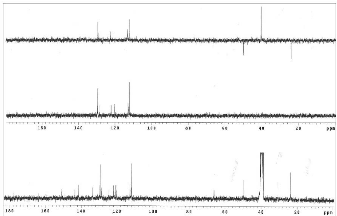
Figure S48. ^{13}\text{C} NMR / DEPT spectra (75.5 MHz, \text{DMSO}-d_6 ) of compound 6c .
