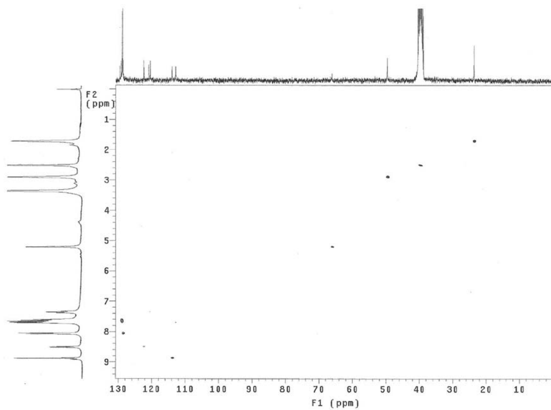
Figure S43. HMQC spectra of compound 6a .
