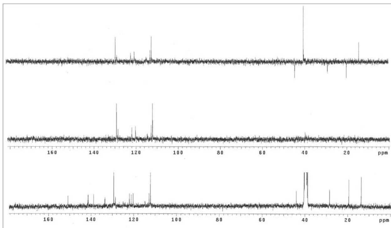
Figure S21. ^{13}\text{C} NMR / DEPT spectra (75.5 MHz, \text{DMSO}-d_6 ) of compound 3c .
