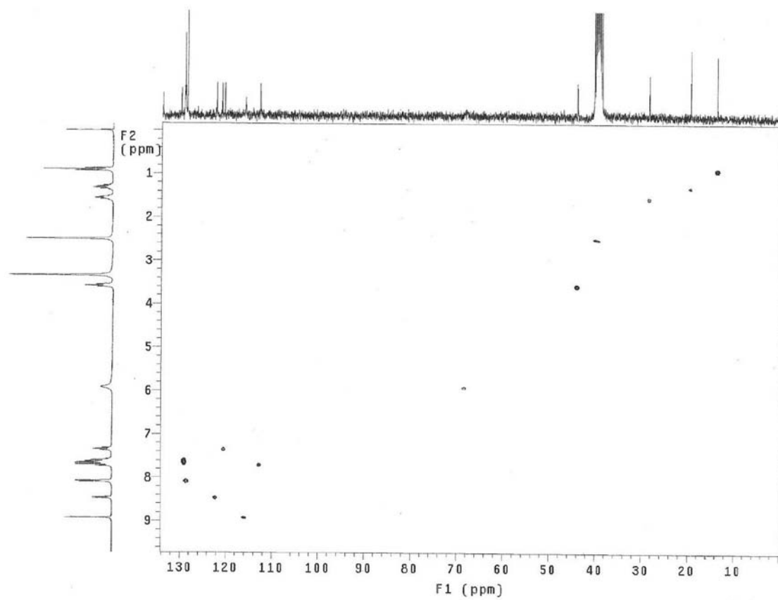
Figure S16. HMBC spectra of compound 3a .
