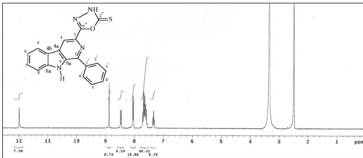
Figure S1. 1 H NMR spectra (300 MHz, DMSO- d 6 ) of compound 1a .
