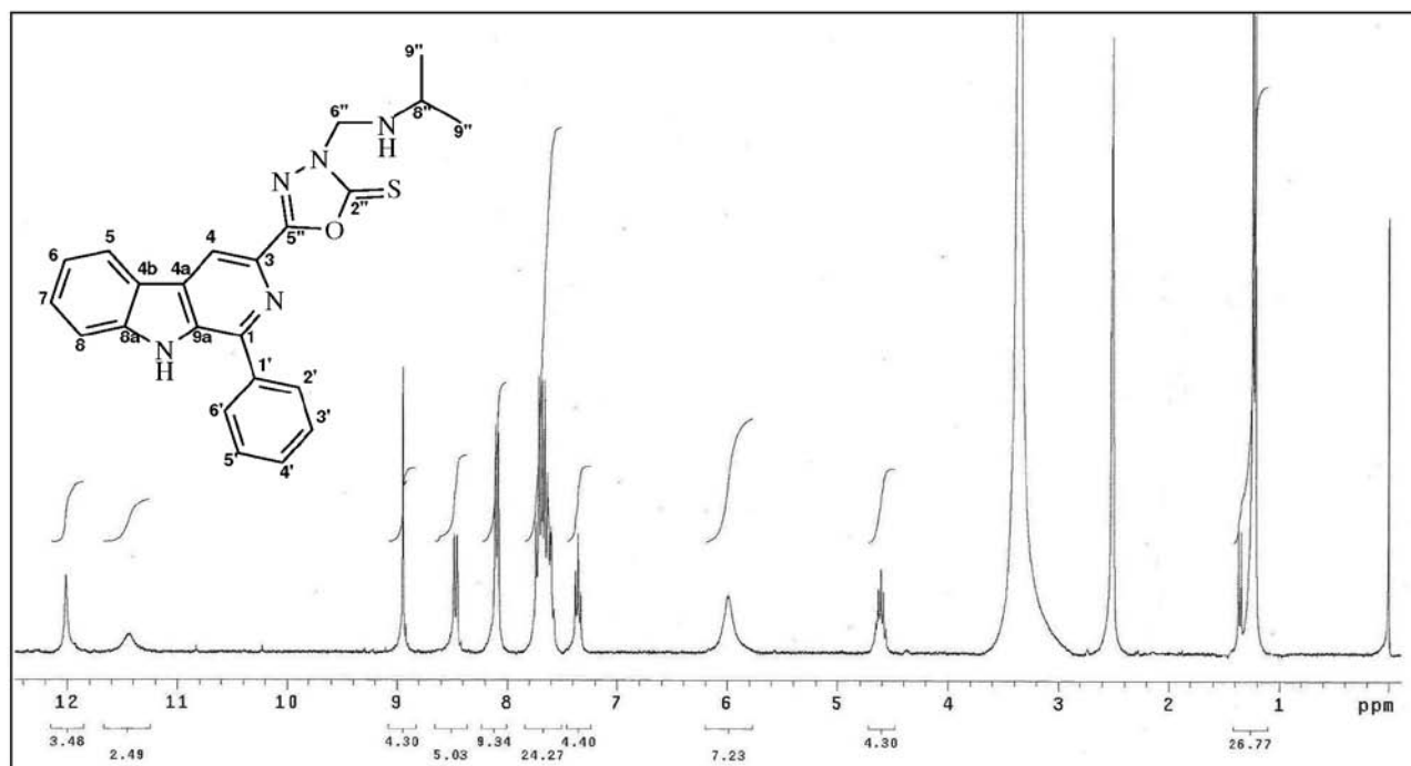
Figure S7. ^1\text{H} NMR spectra (300 MHz, \text{DMSO}-d_6 ) of compound 2a .
