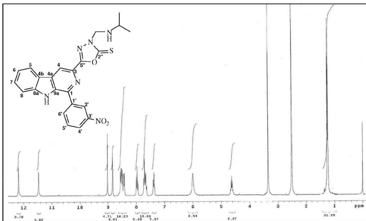
Figure S9. ^1\text{H} NMR spectra (300 MHz, \text{DMSO-}d_6 ) of compound 2b .
