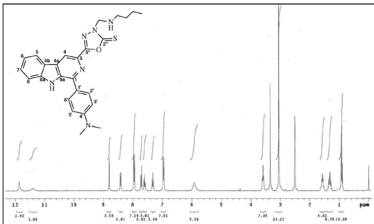
Figure S20. ^1\text{H} NMR spectra (300 MHz, \text{DMSO}-d_6 ) of compound 3c .
