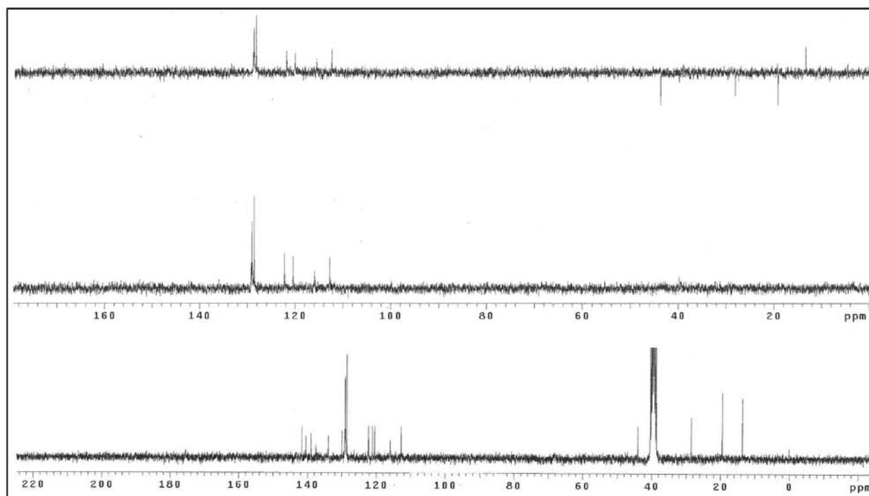
Figure S15. ^{13}\text{C} NMR / DEPT spectra (75.5 MHz, \text{DMSO}-d_6 ) of compound 3a .
