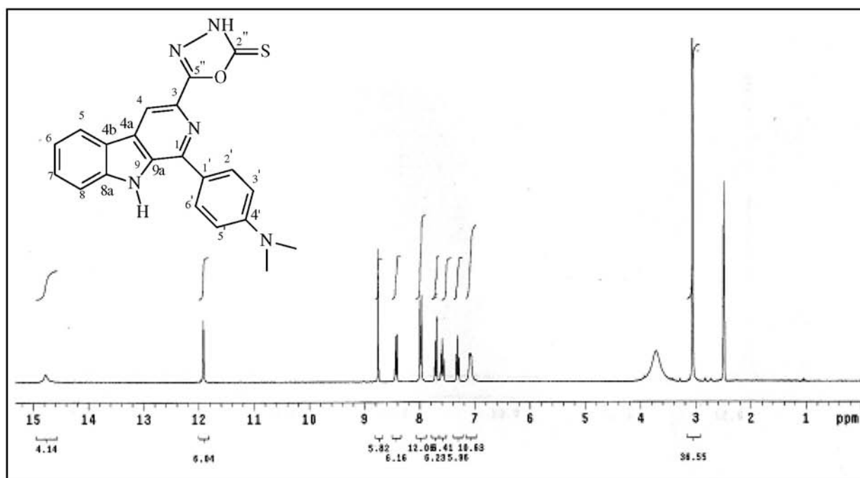
Figure S5. ^1\text{H} NMR spectra (300 MHz, \text{DMSO-}d_6 ) of compound 1c .
