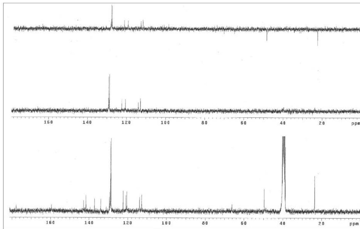
Figure S42. ^{13}\text{C} NMR / DEPT spectra (75.5 MHz, \text{DMSO-}d_6 ) of compound 6a .
