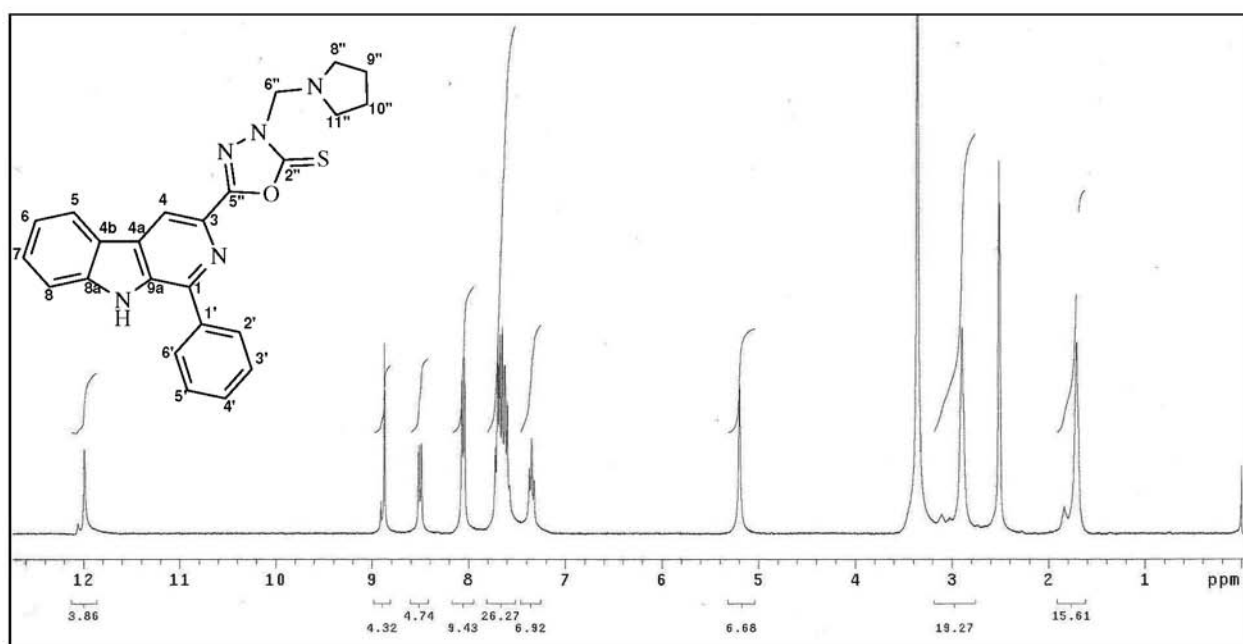
Figure S41. ^1\text{H} NMR spectra (300 MHz, \text{DMSO-}d_6 ) of compound 6a .
