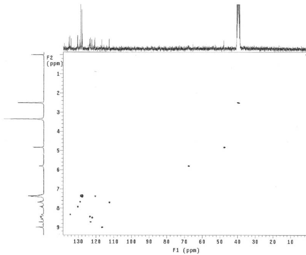
Figure S37. HMQC spectra of compound 5b .
