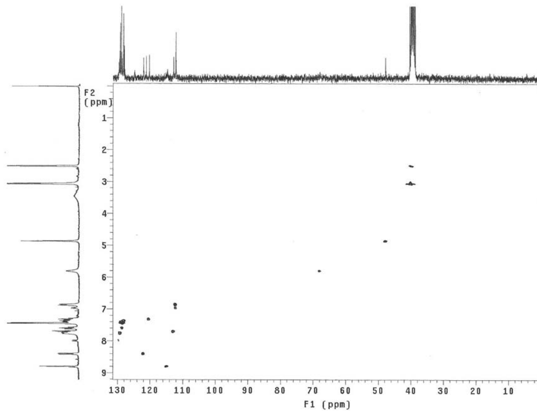
Figure S40. HMQC spectra of compound 5c .
