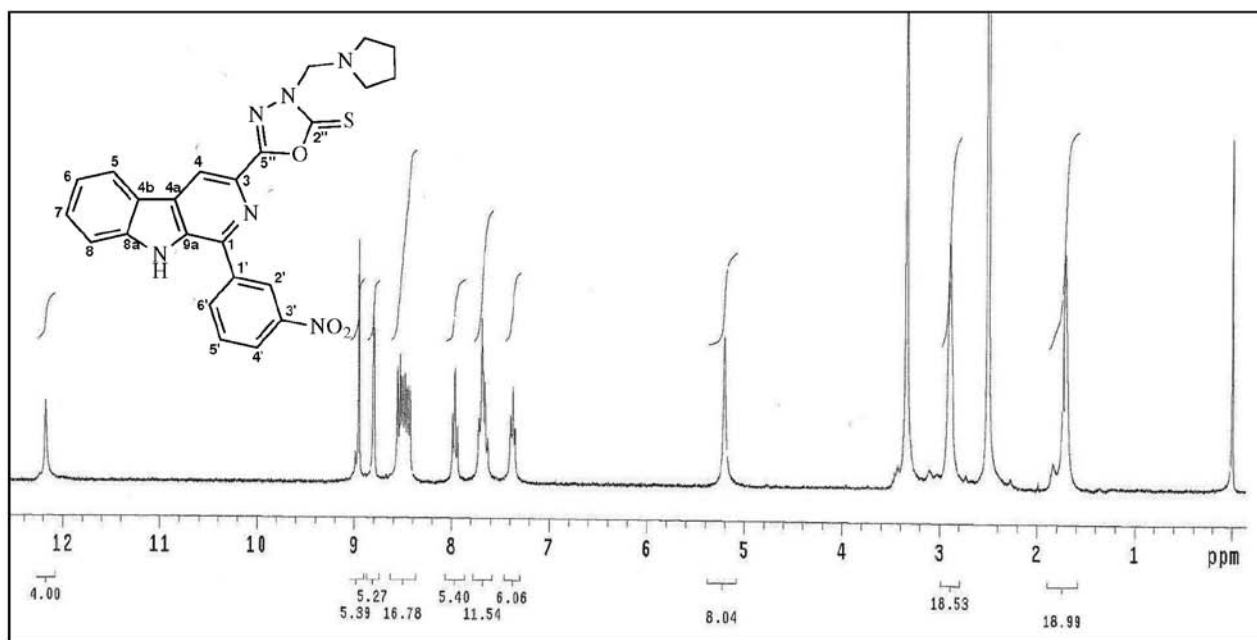
Figure S44. 1 H NMR spectra (300 MHz, DMSO- d 6 ) of compound 6b .
