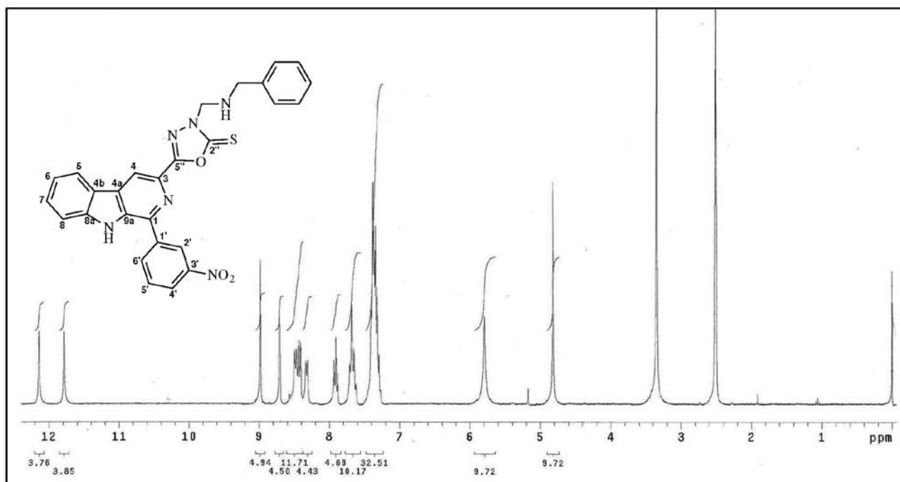
Figure S35. 1 H NMR spectra (300 MHz, DMSO- d 6 ) of compound 5b .
