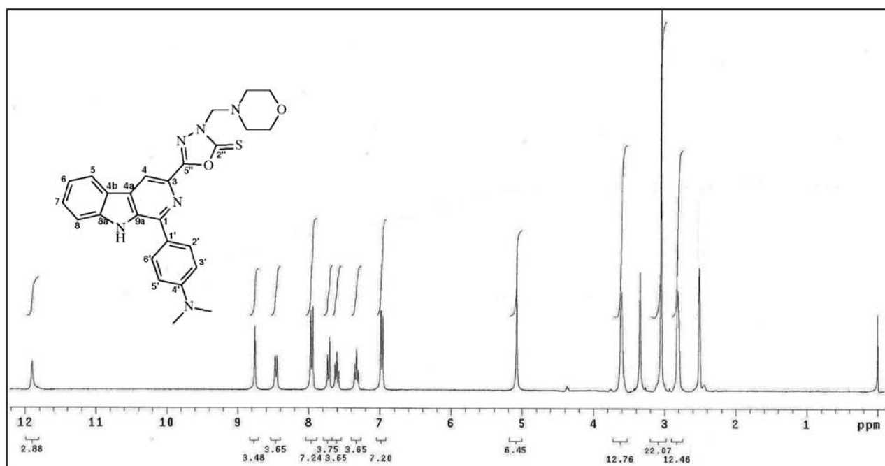
Figure S55. ^1\text{H} NMR spectra (300 MHz, \text{DMSO-}d_6 ) of compound 7c.
