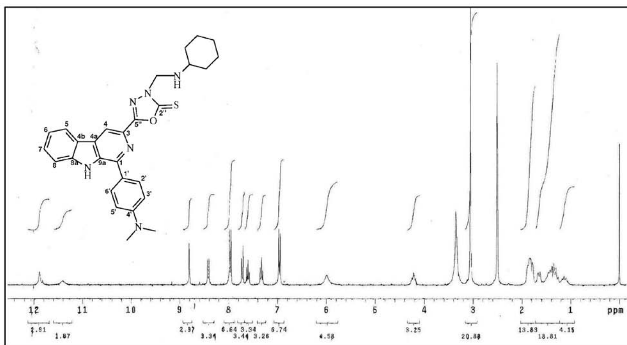
Figure S29. ^1\text{H} NMR spectra (300 MHz, \text{DMSO-}d_6 ) of compound 4c .
