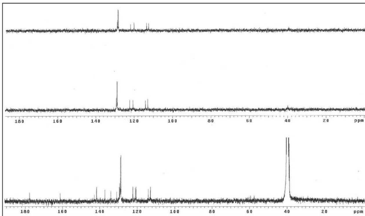
Figure S2. ^{13}\text{C} NMR / DEPT spectra (75.5 MHz, \text{DMSO-}d_6 ) of compound 1a .
