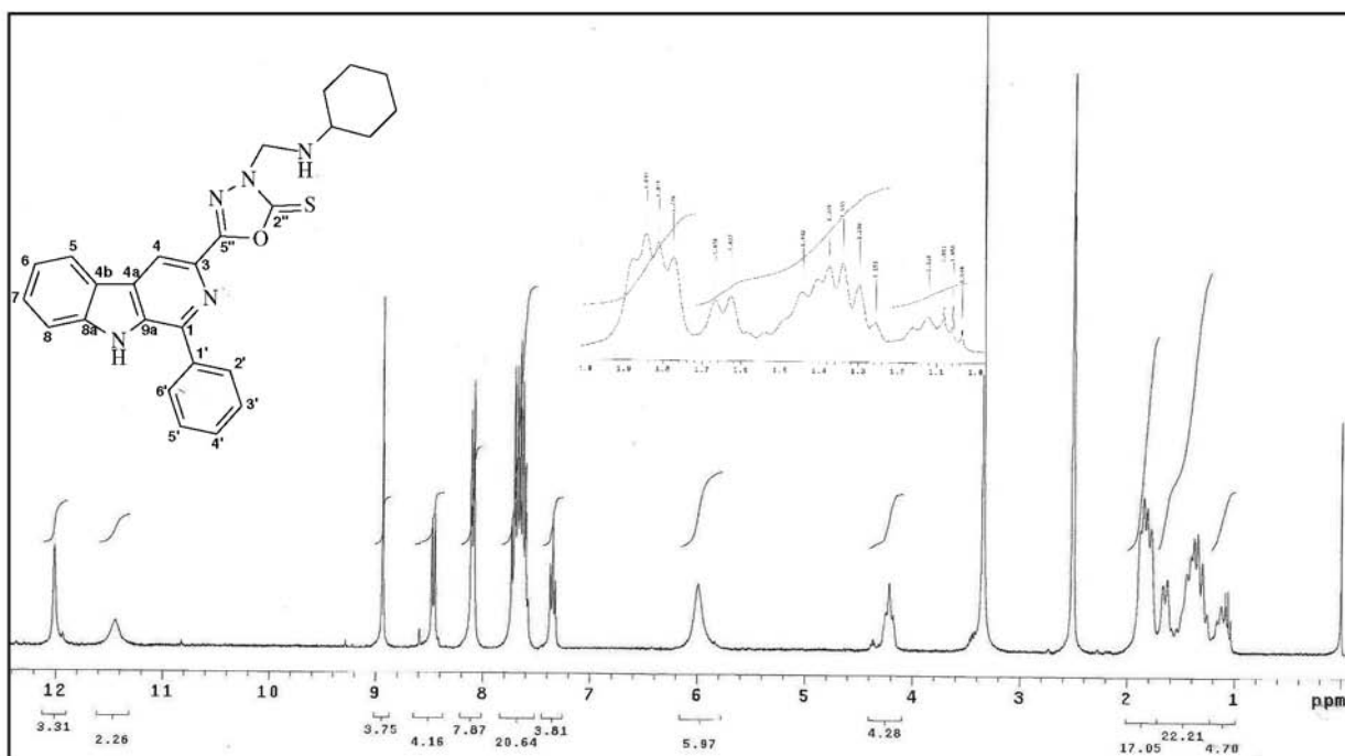
Figure S23. ^1\text{H} NMR spectra (300 MHz, \text{DMSO-}d_6 ) of compound 4a .
