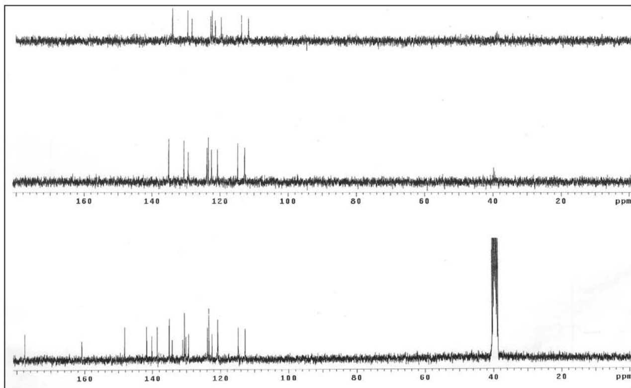
Figure S4. ^{13}\text{C} NMR / DEPT spectra (75.5 MHz, \text{DMSO-}d_6 ) of compound 1b .
