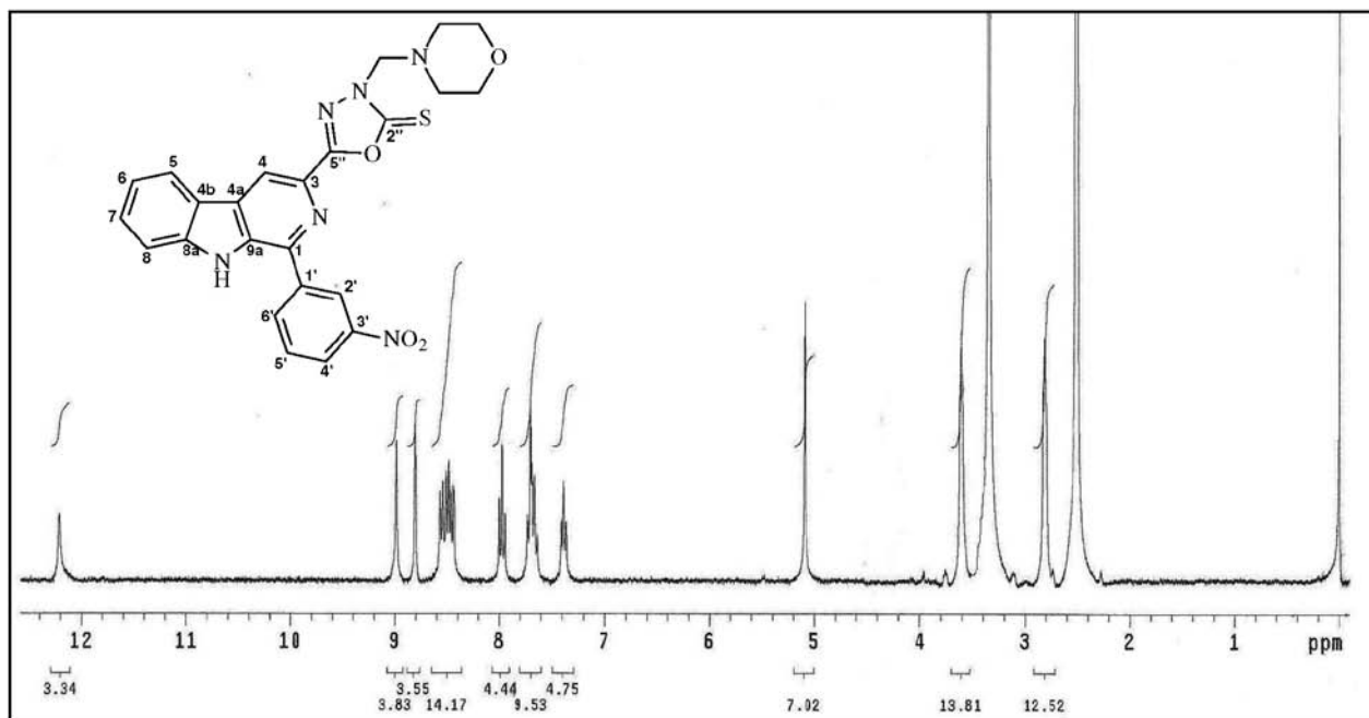
Figure S52. 1 H NMR spectra (300 MHz, DMSO- d 6 ) of compound 7b.
