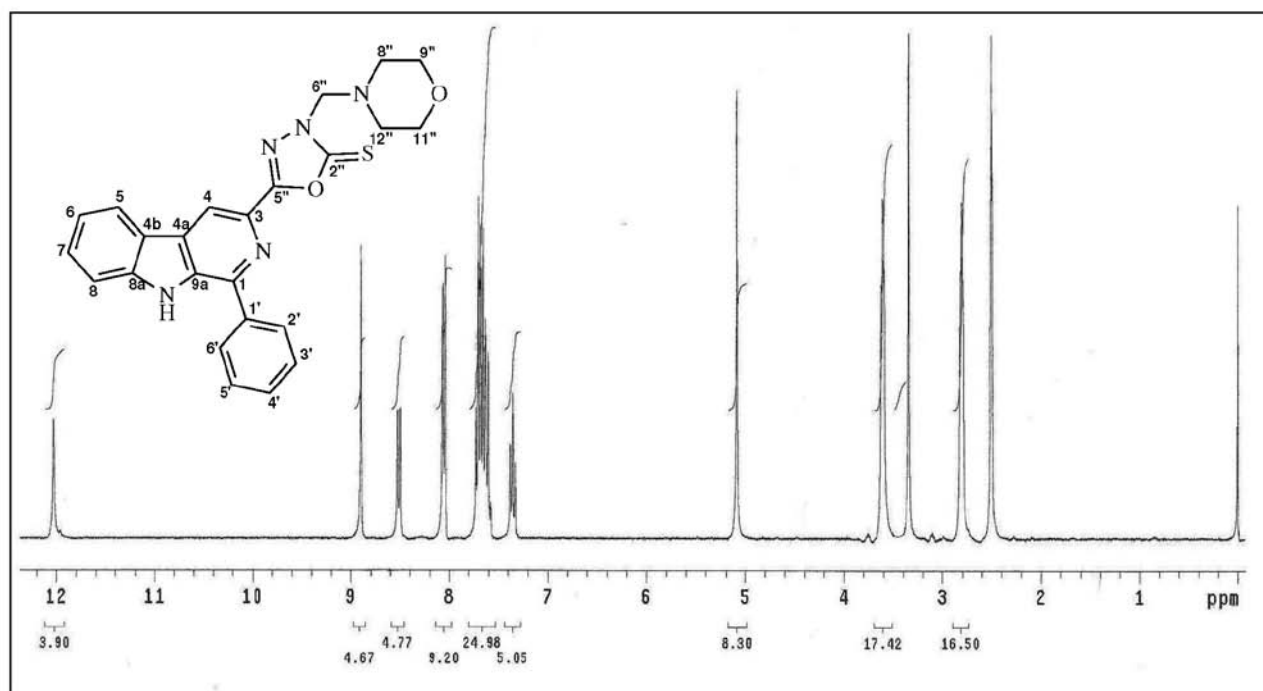
Figure S49. ^1\text{H} NMR spectra (300 MHz, \text{DMSO}-d_6 ) of compound 7a .
