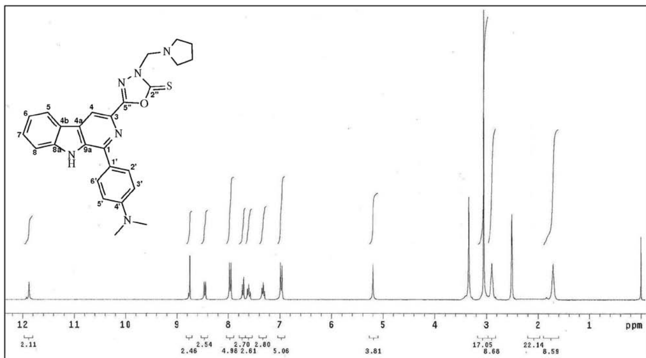
Figure S47. ^1\text{H} NMR spectra (300 MHz, \text{DMSO-}d_6 ) of compound 6c .
