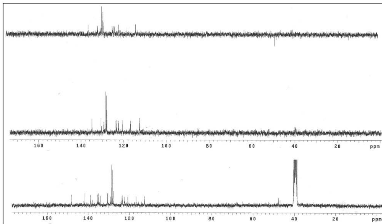
Figure S36. ^{13}\text{C} NMR / DEPT spectra (75.5 MHz, \text{DMSO-}d_6 ) of compound 5b .
