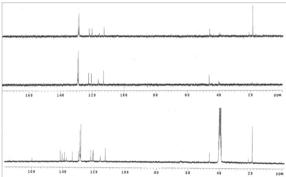
Figure S8. ^{13}\text{C} NMR / DEPT spectra (75.5 MHz, \text{DMSO-}d_6 ) of compound 2a .
