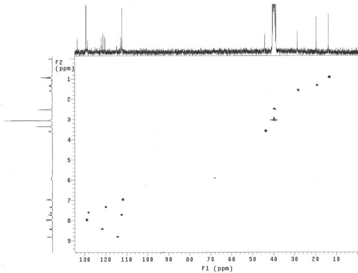
Figure S22. HMOC spectra of compound 3c .
