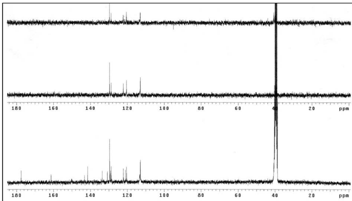
Figure S6. ^{13}\text{C} NMR / DEPT spectra (75.5 MHz, \text{DMSO}-d_6 ) of compound 1c .
