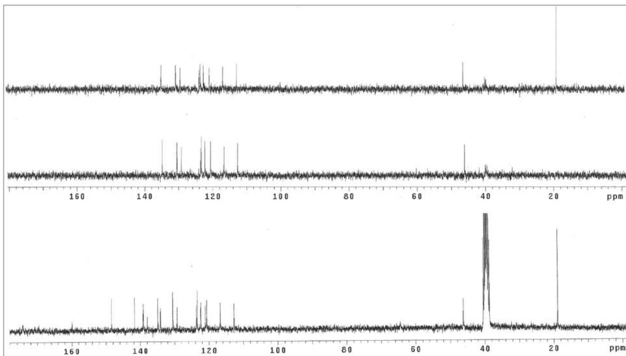
Figure S10. ^{13}\text{C} NMR / DEPT spectra (75.5 MHz, \text{DMSO-}d_6 ) of compound 2b .
