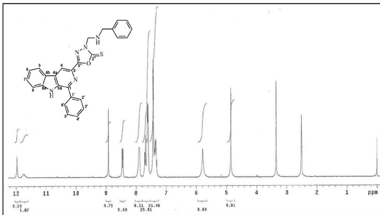
Figure S32. 1 H NMR spectra (300 MHz, DMSO- d 6 ) of compound 5a.
