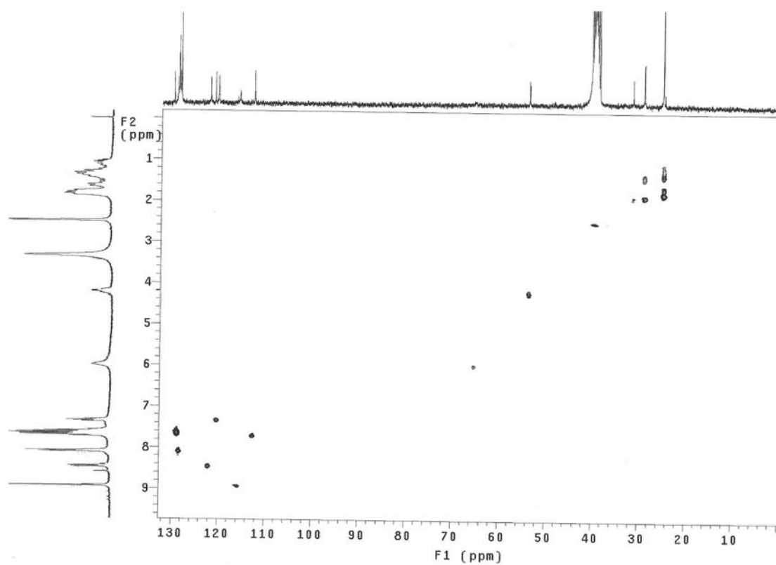
Figure S25. HMQC spectra of compound 4a.
