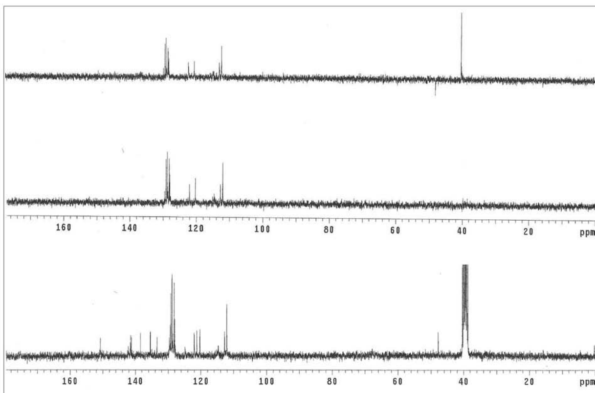
Figure S39. 13 C NMR / DEPT spectra (75.5 MHz, DMSO- d 6 ) of compound 5c.
