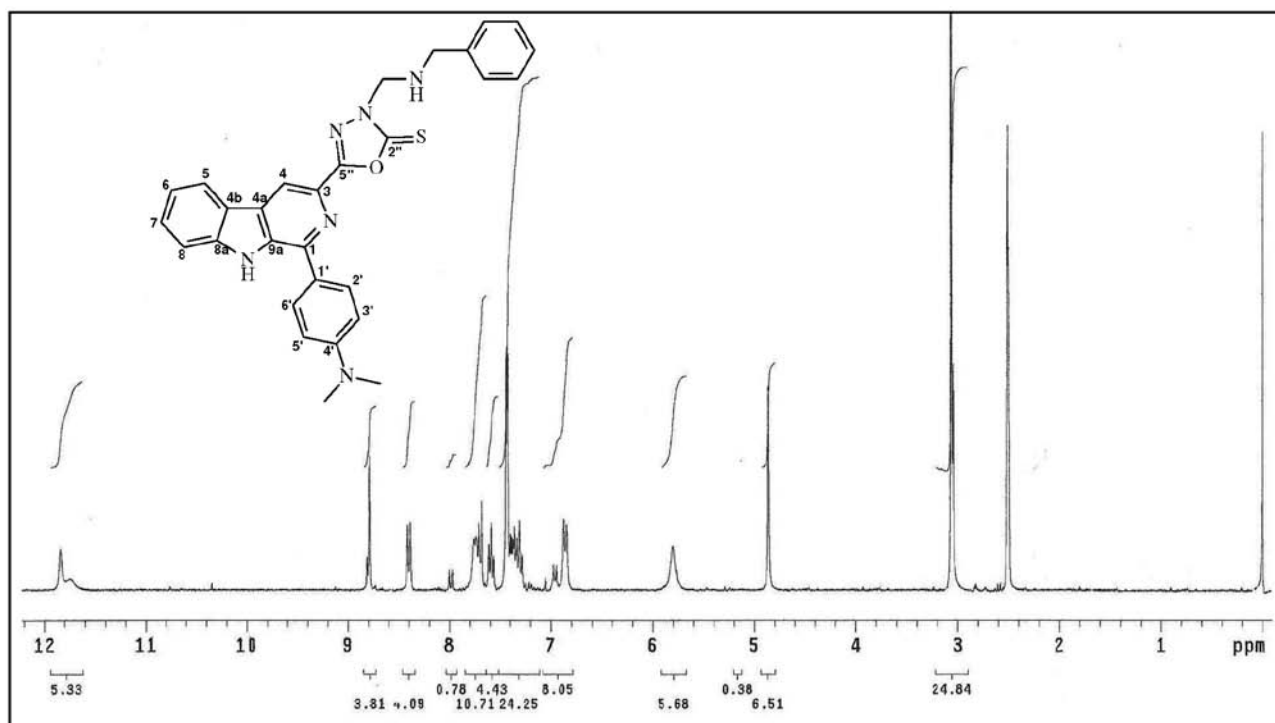
Figure S38. 1 H NMR spectra (300 MHz, DMSO- d 6 ) of compound 5c.
