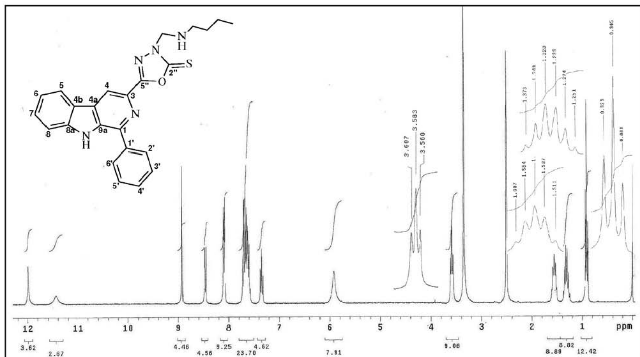
Figure S14. ^1\text{H} NMR spectra (300 MHz, \text{DMSO}-d_6 ) of compound 3a .
