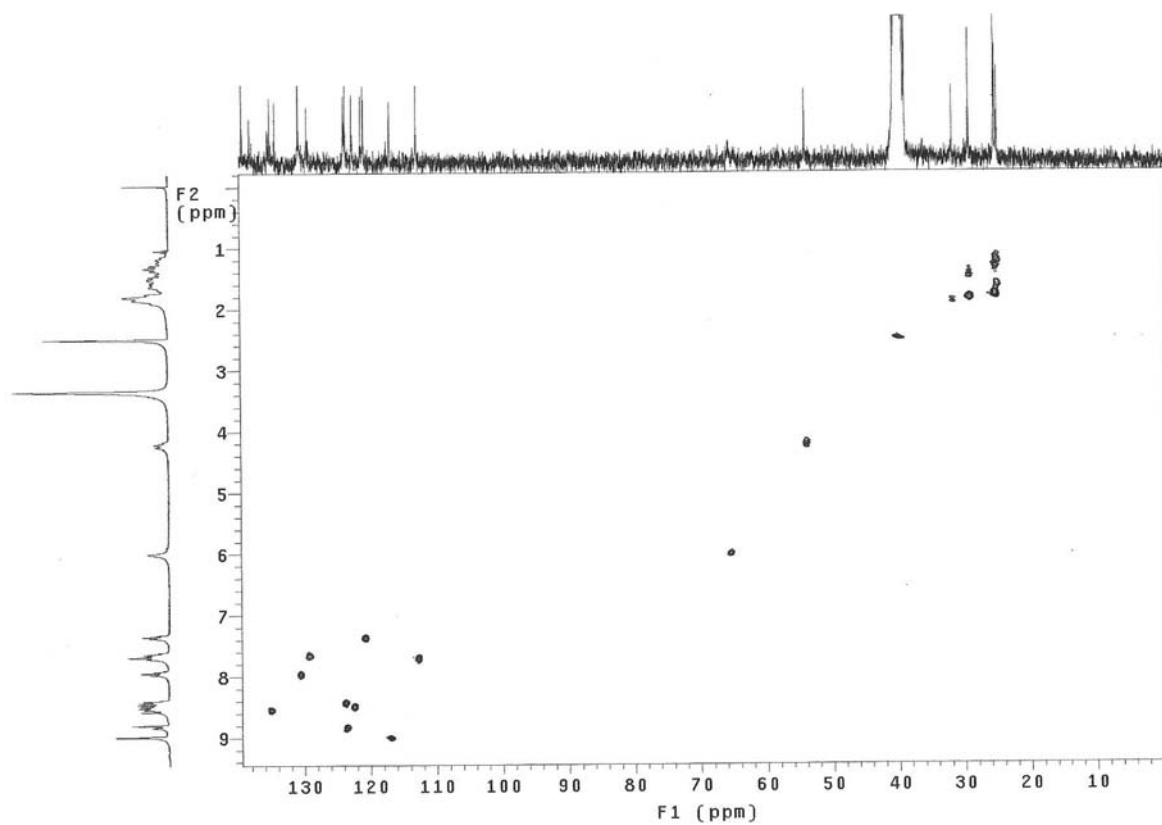
Figure S28. HMQC spectra of compound 4b .
