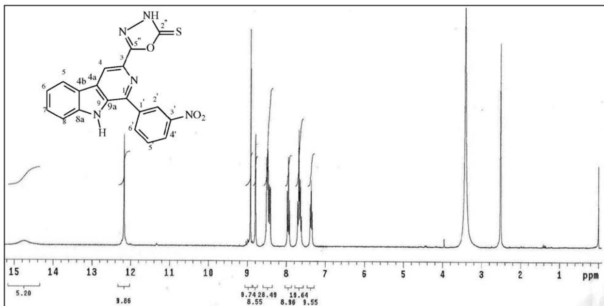
Figure S3. ^1\text{H} NMR spectra (300 MHz, \text{DMSO-}d_6 ) of compound 1b .
