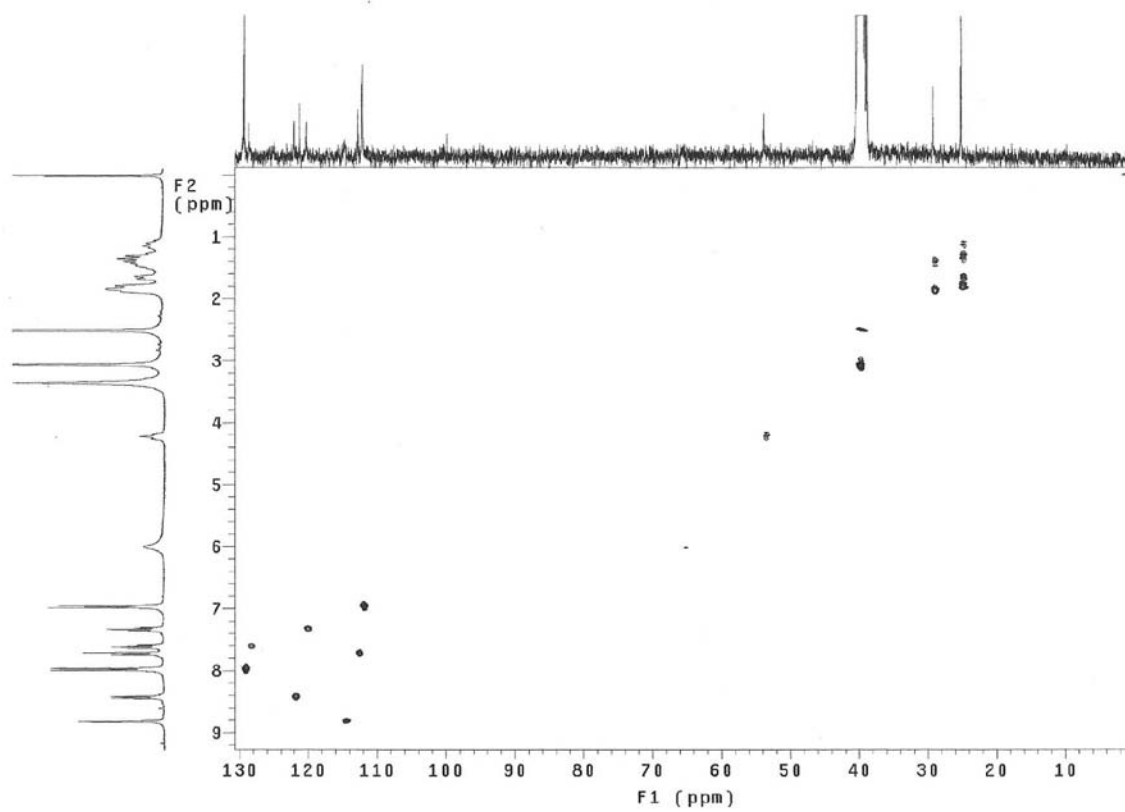
Figure S31. HMQC spectra of compound 4c.
