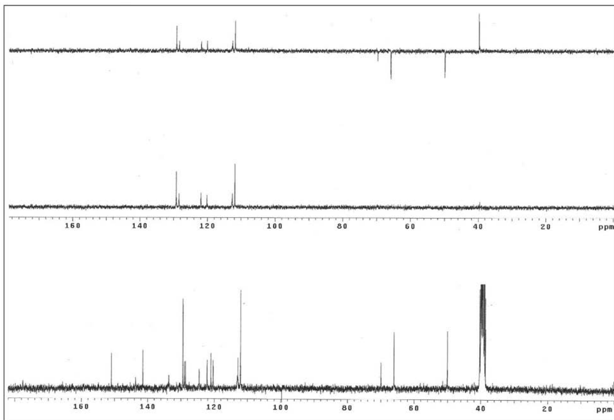
Figure S56. 13 C NMR / DEPT spectra (75.5 MHz, DMSO- d 6 ) of compound 7c.
