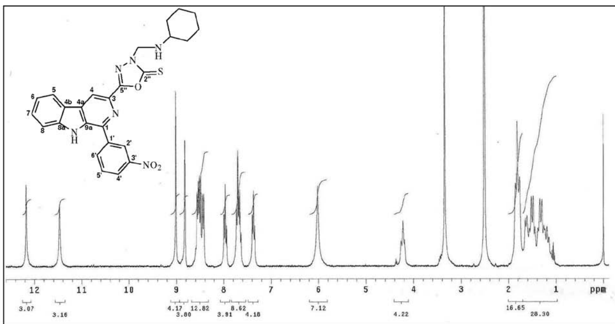
Figure S26. ^1\text{H} NMR spectra (300 MHz, \text{DMSO-}d_6 ) of compound 4b .
