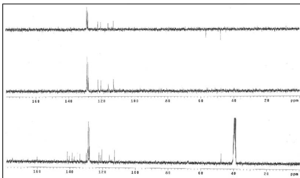
Figure S33. 13 C NMR / DEPT spectra (75.5 MHz, DMSO- d 6 ) of compound 5a.
