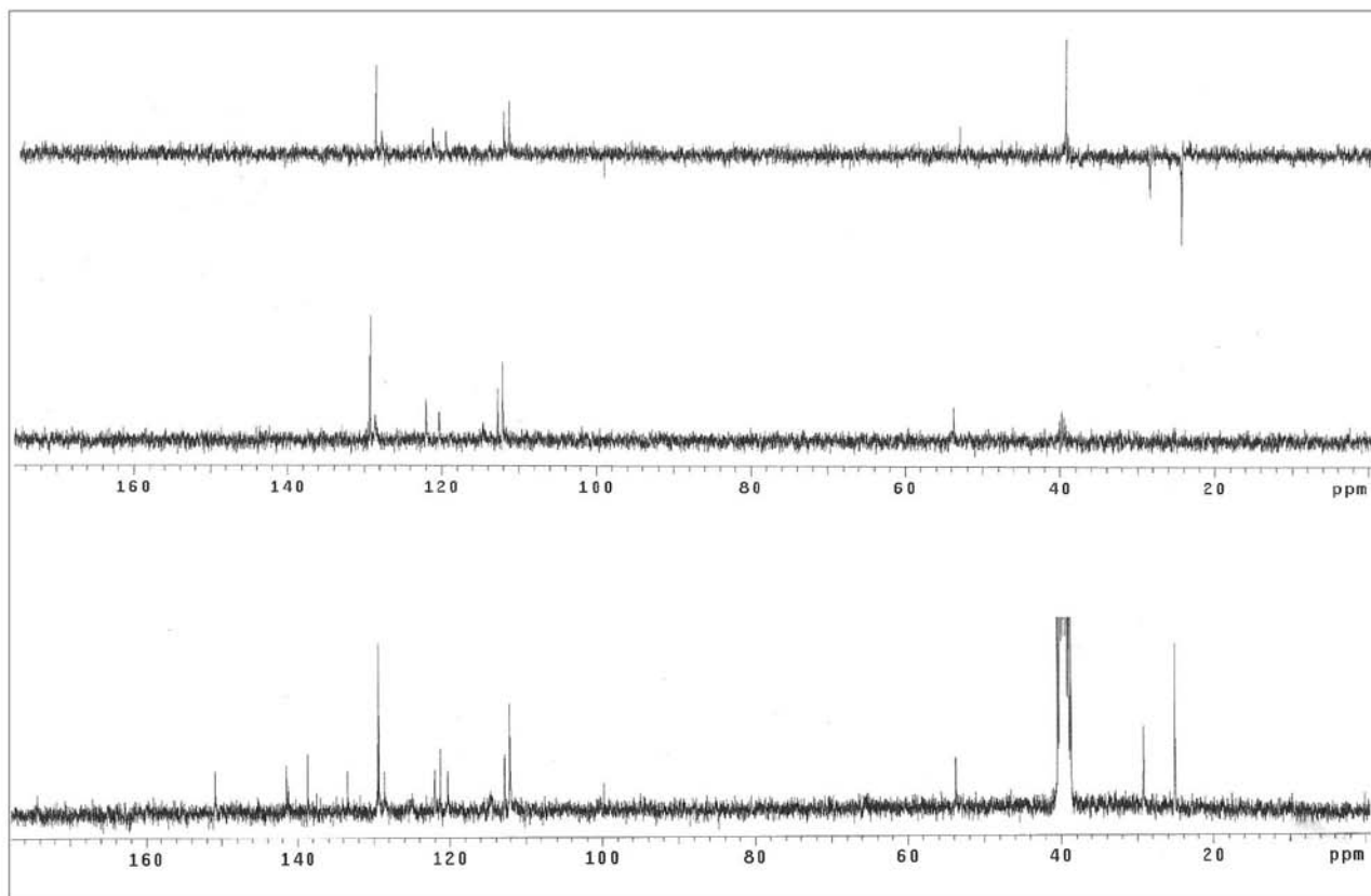
Figure S30. ^{13}\text{C} NMR / DEPT spectra (75.5 MHz, \text{DMSO-}d_6 ) of compound 4c.
