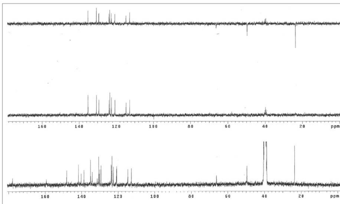
Figure S45. 13 C NMR / DEPT spectra (75.5 MHz, DMSO- d 6 ) of compound 6b .
