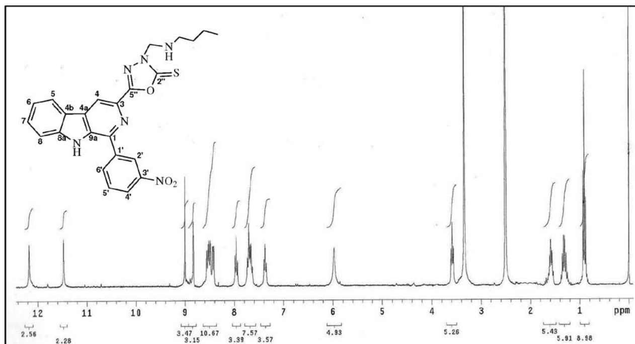
Figure S17. ^1\text{H} NMR spectra (300 MHz, \text{DMSO-}d_6 ) of compound 3b .
