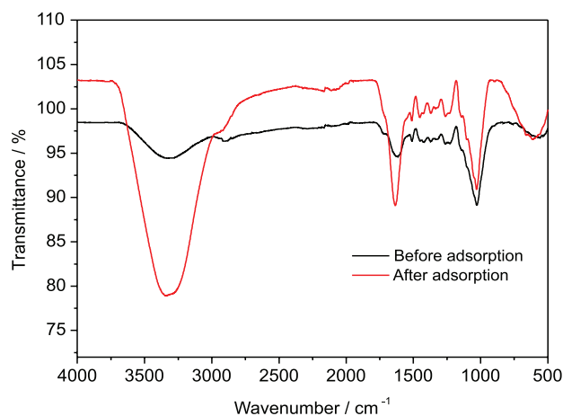
Figure 1. FTIR spectra before and after Cr^{VI} biosorption.
