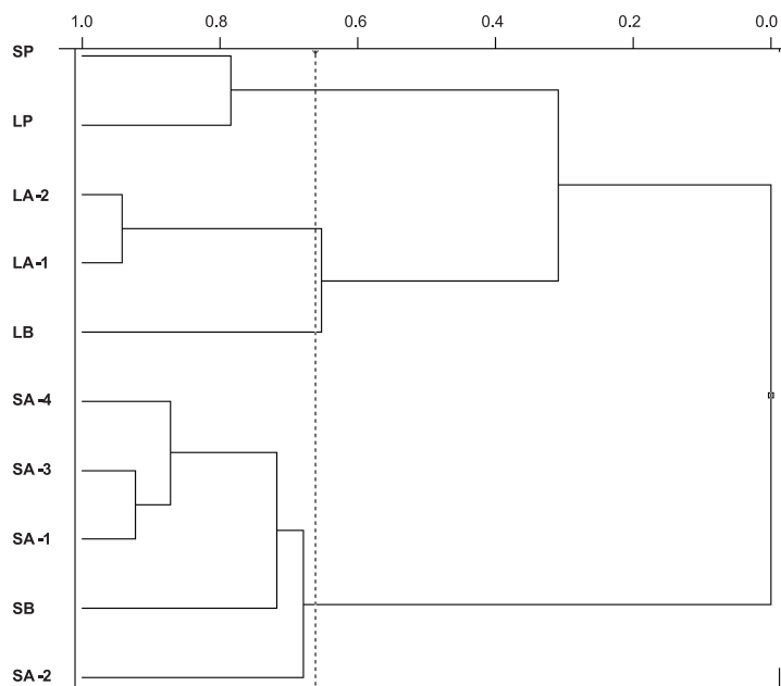
Figure 2. Dendrogram constructed following agglomerative hierarchical clustering analysis (HCA) of essential oils of A. giberti of different provenances and collection dates.
