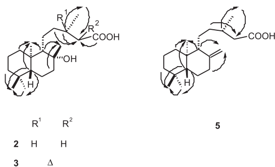
Figure 5. Selected gHMBC correlations (→) for diterpenes 2 , 3 , and 5 .
