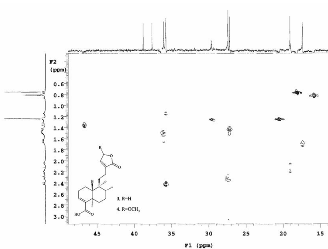
Figure S27. HMBC NMR experiment (CDCl 3 , 500 x 125 MHz, \delta_c 15-45) of the compounds 3 and 4 isolated of Nanuza plicata .
