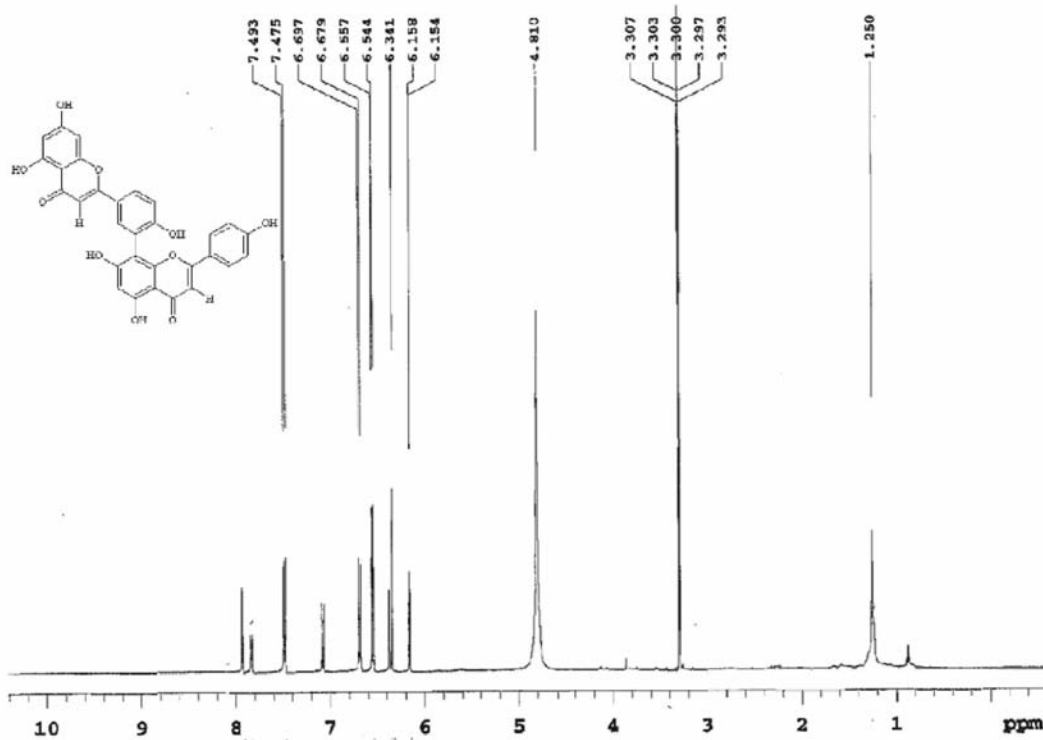
Figure S17. 1 H NMR spectrum (CD 3 OD, 500 MHz) of the compound 2 isolated of Nanuza plicata .
