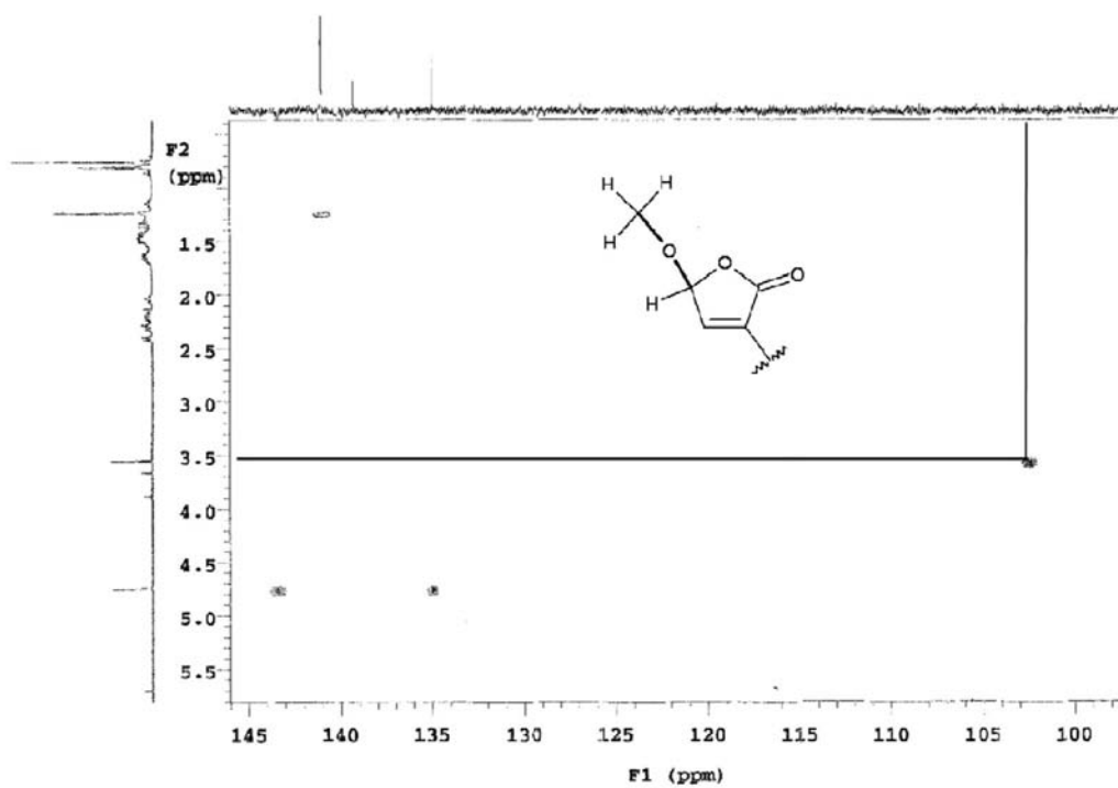
Figure S28. HMBC NMR experiment ( \text{CDCl}_3 , 500 x 125 MHz, \delta_C 100-145) of the compounds 3 and 4 isolated of Nanuza plicata . * Correlation of compounds 4 .
