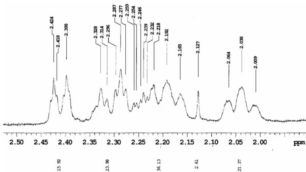
Figure S24. 1 H NMR spectrum (CDCl 3 , 500 MHz, δ H 2.0-2.4) of the compounds 3 and 4 isolated of Nanuza plicata .
