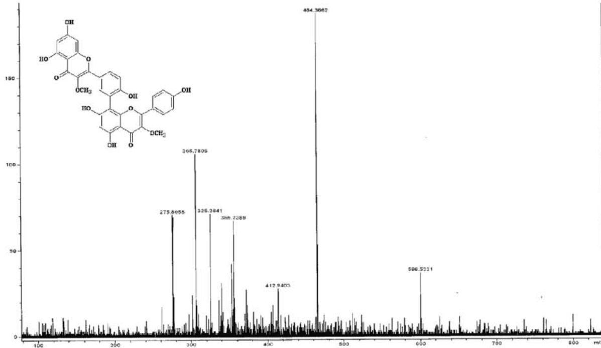
Figure S5. HR-ESI-MS spectrum of the compound 1 isolated of Nanuza plicata .
