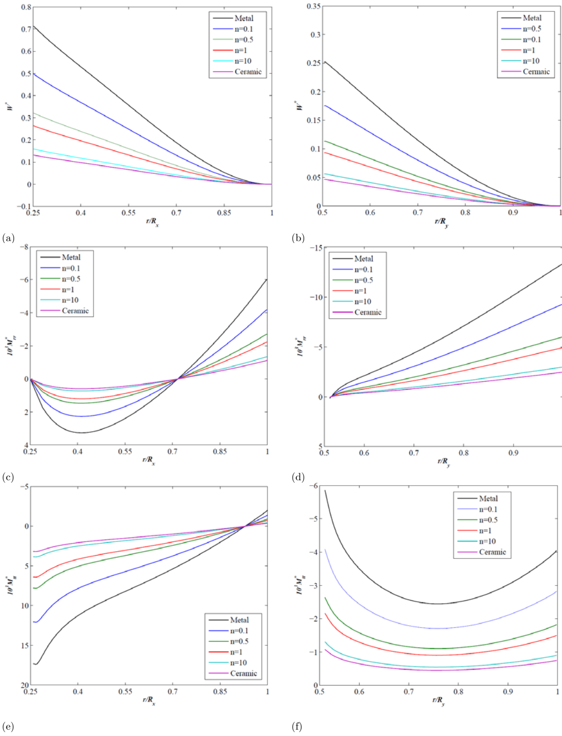
Figure 9 Non-dimensional deflection w^* and resultant moments M_{rr}^*, M_{tt}^* along semi-major (a, c, e) and semi-minor axes (b, d, f) of free-clamped FG elliptic plate with various powers of FGM ( \frac{R_x}{R_y} = 2, \frac{R_z}{R_t} = 4 ).
