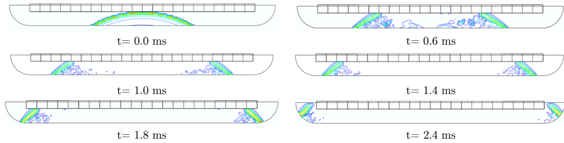
Figure 10 The propagation of shock wave
