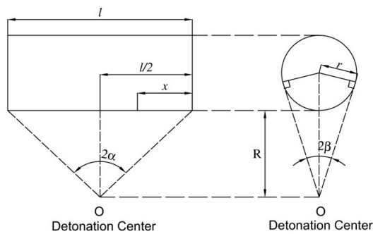
Figure 1 Loading geometry as demonstrated in [5]
