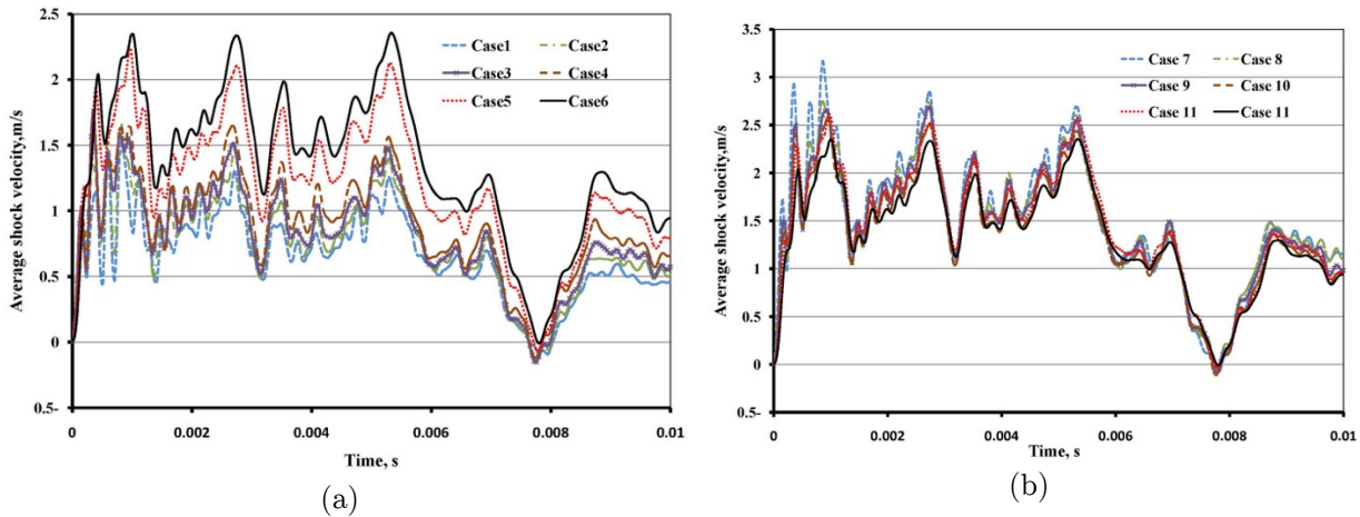
Figure 8 Average shock spectrum velocity for a) C_1 = 0.104 ; b) C_2 = 2.149
