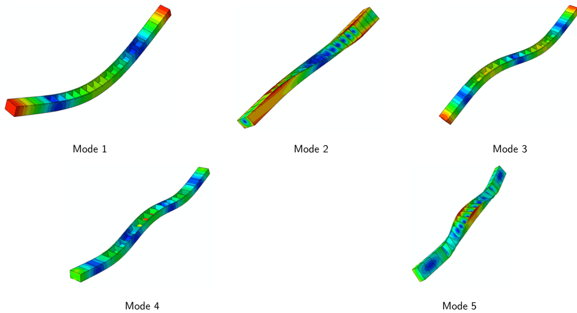
Figure 4 Mode shapes of scaled ship model
