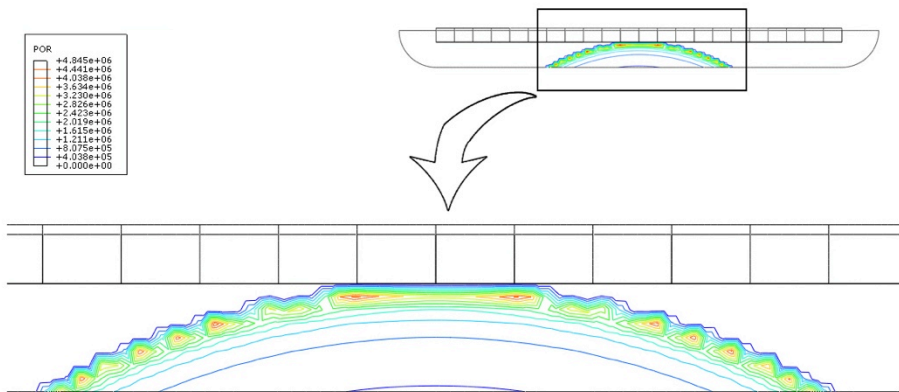
Figure 5 Pressure profile in the fluid domain, near the fluid-structure interface (for 0.5 kg TNT and stand-off 6 m)
