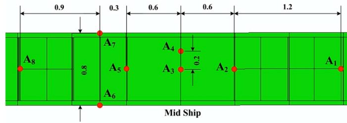
Figure 6 Points adopted on the structure bottom surface (all dimensions are in meter)
