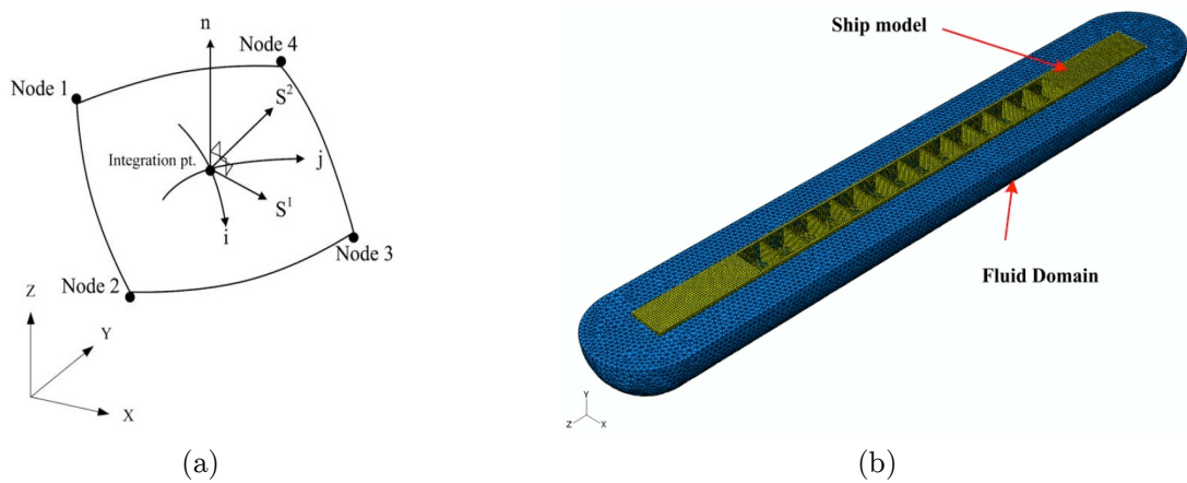
Figure 3 Finite element model a) 4-node shell element, S4R; b) FE model
