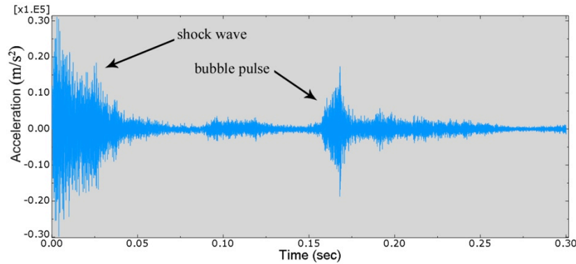
Figure 7 Acceleration of point A 1 (0.5 kg exactly under the structure at the stand-off of 6 m)
