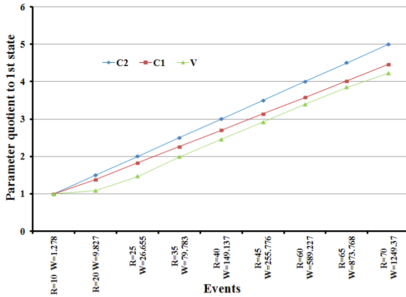
Figure 9 Average shock velocity, C_1 and C_2
