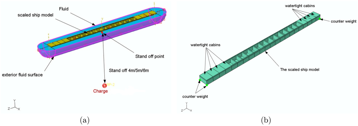
Figure 2 Scaled Ship models: a) Attack geometry surrounded by fluid media; b) Basic structure
