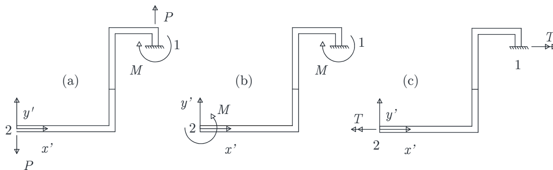
Figure 2: Lead free-body diagrams: (a) concentrated lead P ; (b) bending moment M ; (c) torsional moment T .
