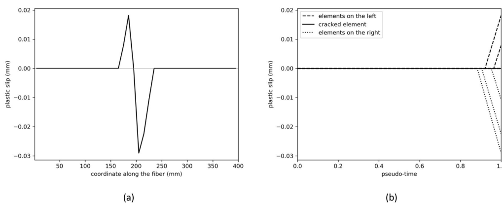
Figure 8: Plastic slip: (a) distribution of \alpha^{bs,p} along the reinforcement bar at the end of the analysis (values at Gauss points); (b) evolution in time for the enriched elements that have entered the plastic phase.
