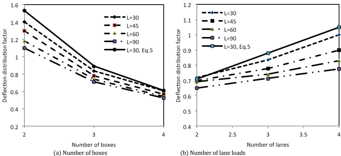
Figure 11 Effect of different Parameters on Distribution Factor of Deflection
