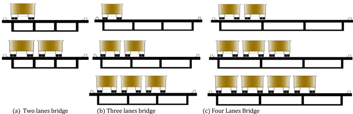
Figure 5 LRFD HL93 loading cases in the transverse direction of the bridges for two, three and four lane loading
