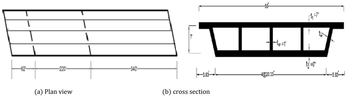
Figure 4 Plan View and Cross Section of Bridge No. 14 of comparative model (Huo et al., 2003)
