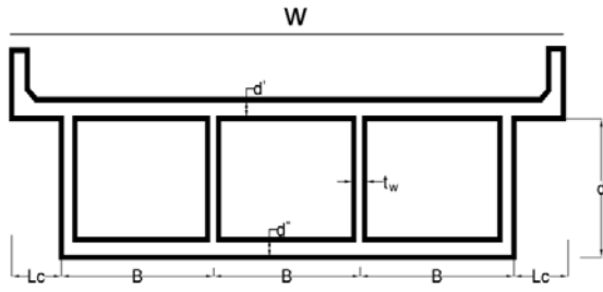
Figure 1 Cross Section Symbols for three Boxes Bridge
