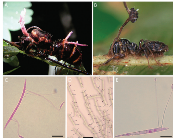
Fig. 2: spore form and function in the zombie-ant fungus, Ophiocordyceps unilateralis sensu lato ; all collected at the same time and from the same locality as specimens in Fig. 1; (A) zombie-ant queen of Camponotus species, dying with its mandibles embedded in foliage of forest shrub and immature fungal structures emerging from sutures of upper neck and abdominal regions; (B) zombie-ant worker of a different species of Camponotus in a similar biting position, with mature sexual stage (ascostroma) emerging; (C-E) germinating ascospores, producing specialised needle-like outgrowths (capillispores) with sticky capillispores, analogous to the germination process in the Entomophthorales ; note the ascospores deposited on a glass slide, producing rows of sticky 'traps' to attach to passing ants (D). Bars = 10 \mu m, except E = 30 \mu m.
