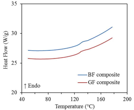
Figure 2. DSC curves for BF and GF composites.
