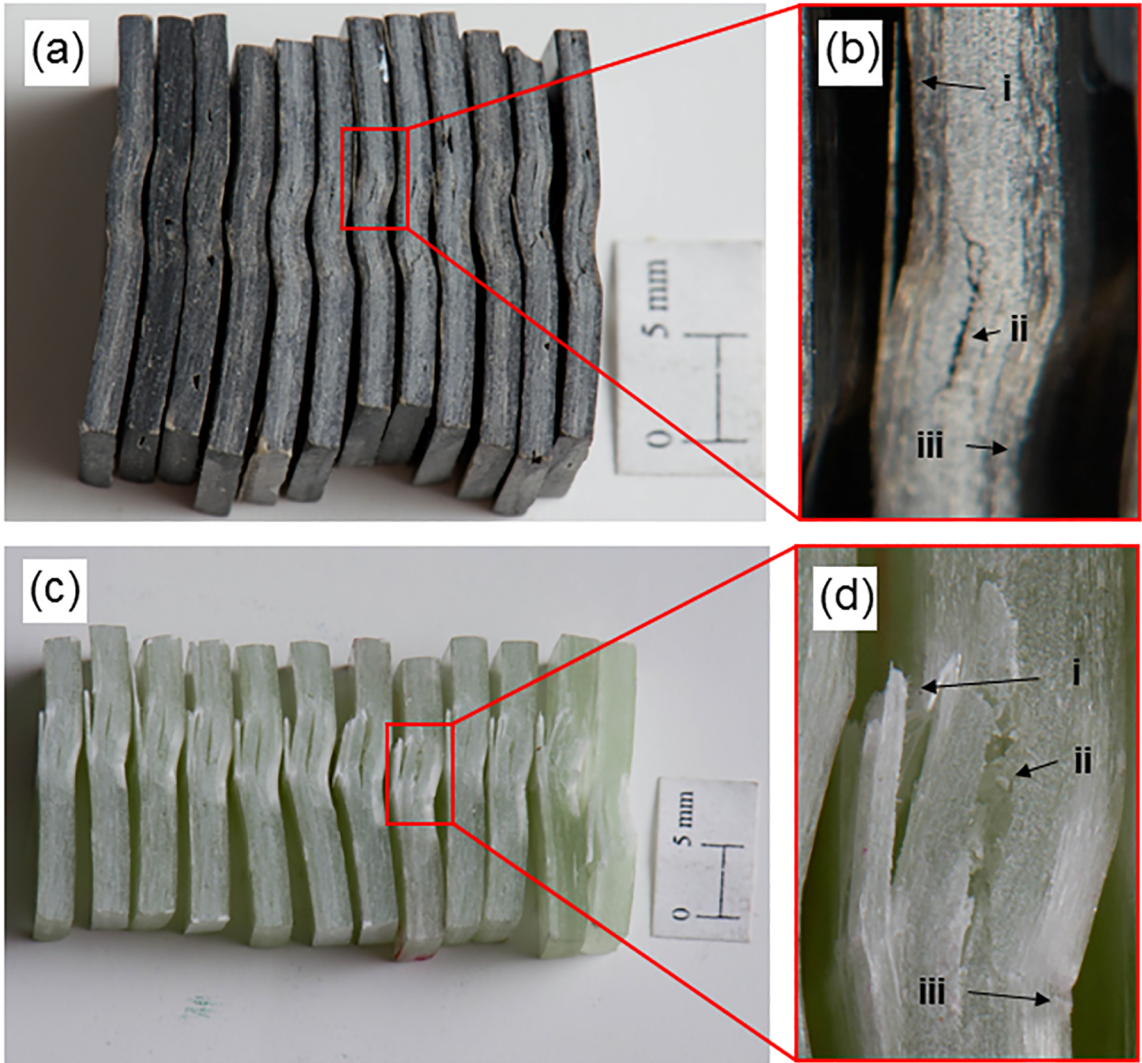
Figure 3. Aspect of (a) BF and (c) GF composite specimens after ILSS test. Identification of failure modes in (b) BF and (d) GF specimens; (i) tension failure, (ii) interlaminar shear, (iii) inelastic deformation.
