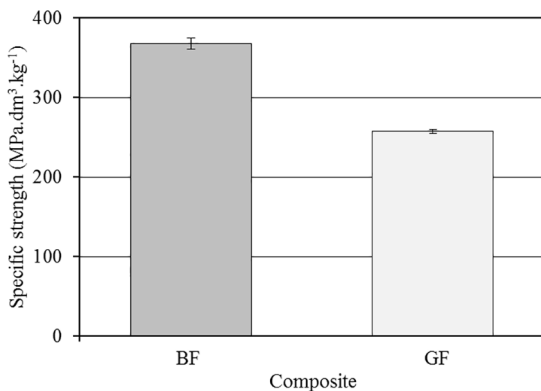
Figure 9. Comparison of ring tensile specific strength between BF and GF composites (mean values).
