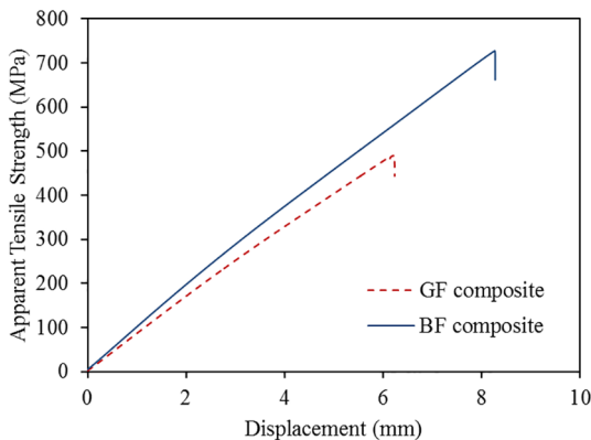
Figure 6. Split disk test tensile-displacement curves of BF and GF composites.
