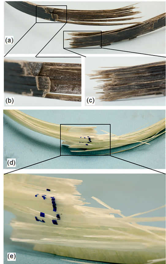
Figure 7. (a) BF and (d) GF ring segment specimen failure. Detail view of (b, c) BF and (e) GF specimens.
