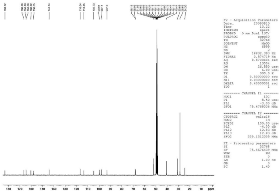
Figure 41S. ^{13}\text{C} NMR spectrum of (15), 75 MHz, methanol- d_4 .
