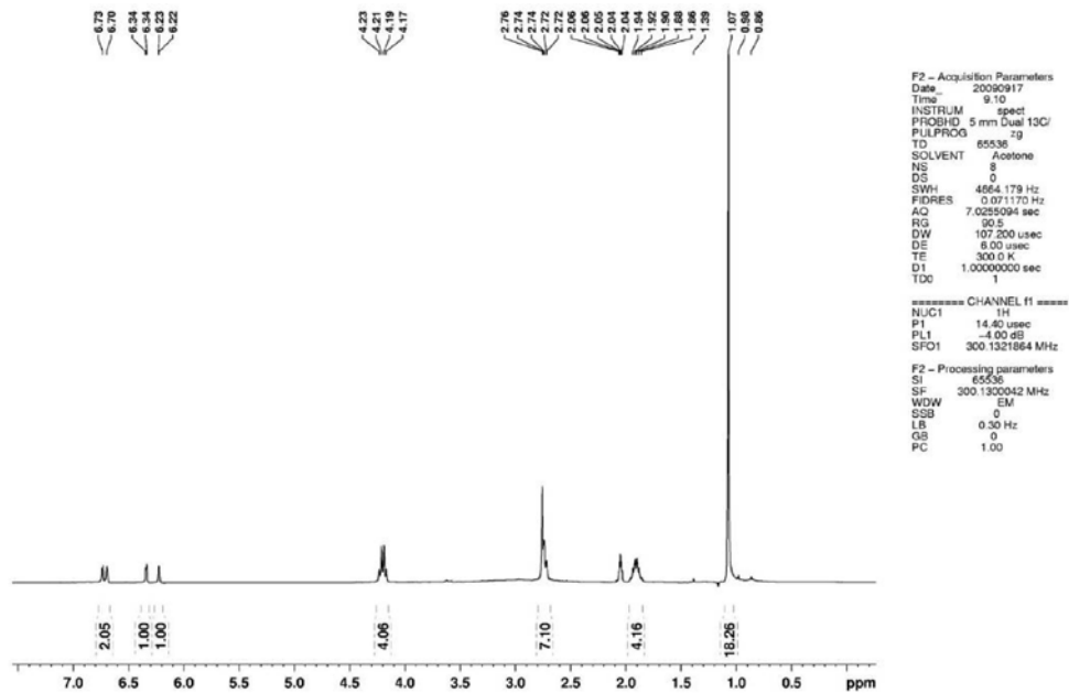
Figure 40S. ^1\text{H} NMR spectrum of (15), 300 MHz, acetone- d_6 .
