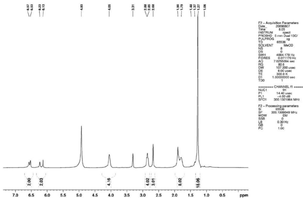
Figure 43S. ^1\text{H} NMR spectrum of (16), 300 MHz, methanol- d_4
