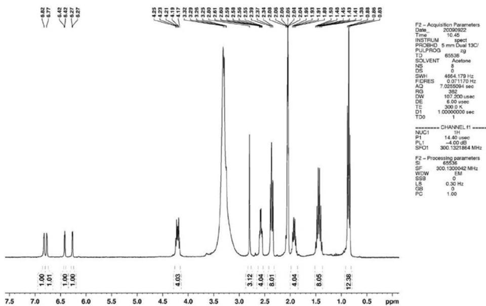
Figure 27S. ^1\text{H} NMR spectrum of (12), 300 MHz, acetone- d_6 /methanol- d_4
