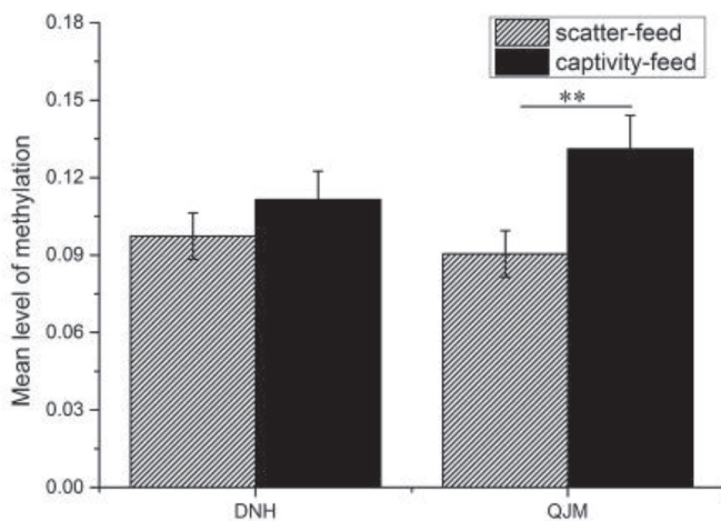
Figure 2 – Mean methylation level of the FATP1 gene in SFDNH, CFDNH, SFQJM and CFQJM chickens
