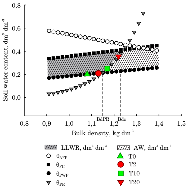
Figure 2. Variation in the Least Limiting Water Range (LLWR) and Available Water (AW) as a function of bulk density (Bd) observed in a distroferic Red Latosol planted to sugarcane in the Brazilian Cerrado. T 0 = 0, T 2 = 2, T 10 = 10 and T 20 = 20 tractor passes in the same place. Bd PR : Bd at the lower limit of the LLWR as limited by θ PR . Bd C : bulk density critical for plant development.
