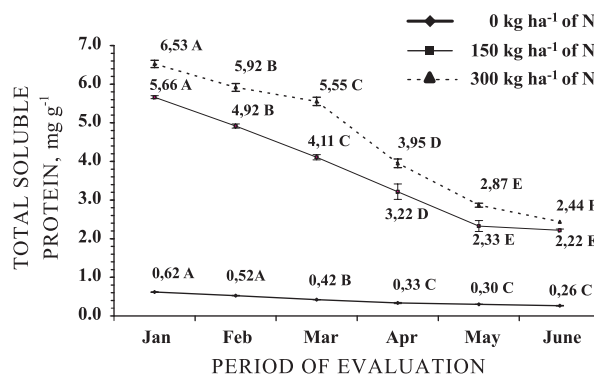
Figure 6. Leaf total soluble protein concentration during the fruit development stadium, considering different N-rates (control, 150 and 300 kg ha -1 ). Means followed by the same letter do not differ by the Tukey test (0.05).
