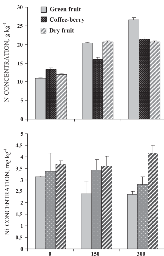
Figure 4. Fruit N and Ni concentrations in different phenological stages, considering different N-rates (control, 150 and 300 kg ha -1 ). Vertical bars indicate mean standard deviations.
