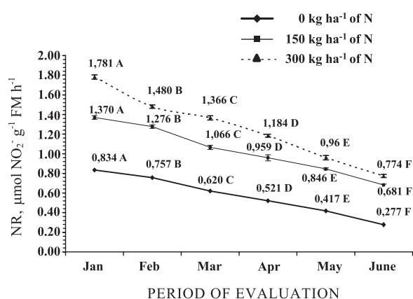
Figure 2. Nitrate reductase activity during fruit development, considering different N-rates (control, 150 and 300 kg ha -1 ). Means followed by the same letter do not differ by the Tukey test (0.05).
