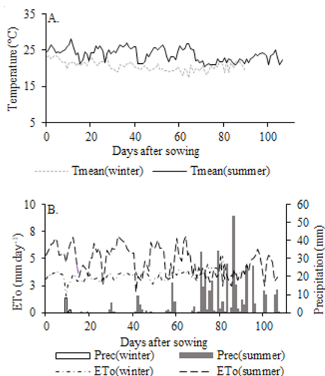
Figure 1. Mean air temperature (Tmean) (A) and reference evapotranspiration (ET o ) and daily precipitation (B) in winter and summer experiments
