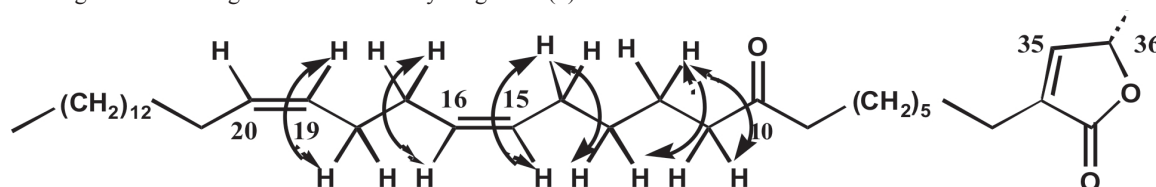
Figure 1. Diagnostic eims fragmentation ions of xymarginatin (1).
