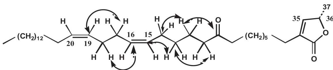
Figure 3. A. ^1\text{H} - ^1\text{H} correlations in the COSY-NMR spectrum of xymarginatin; B. ^1\text{H} - ^{13}\text{C} correlations in the HMBC-NMR spectrum of xymarginatin.
