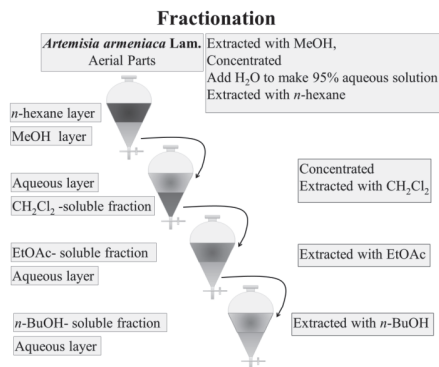
Fig. 1 - Partitioning scheme of n -hexane, \text{CH}_2\text{Cl}_2 , EtOAc, n -BuOH and H 2 O fractions obtained from the crude methanolic extract of Artemisia armeniaca .
