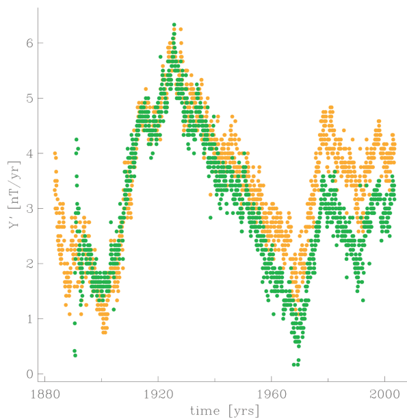
Figure 2 – Secular variation of East component of Chambon la Forêt observatory in France (yellow circles) and Niemeck observatory in Germany (green circles). The data shown are first differences of observatory monthly means that have been smoothed by a 12-month running average.
