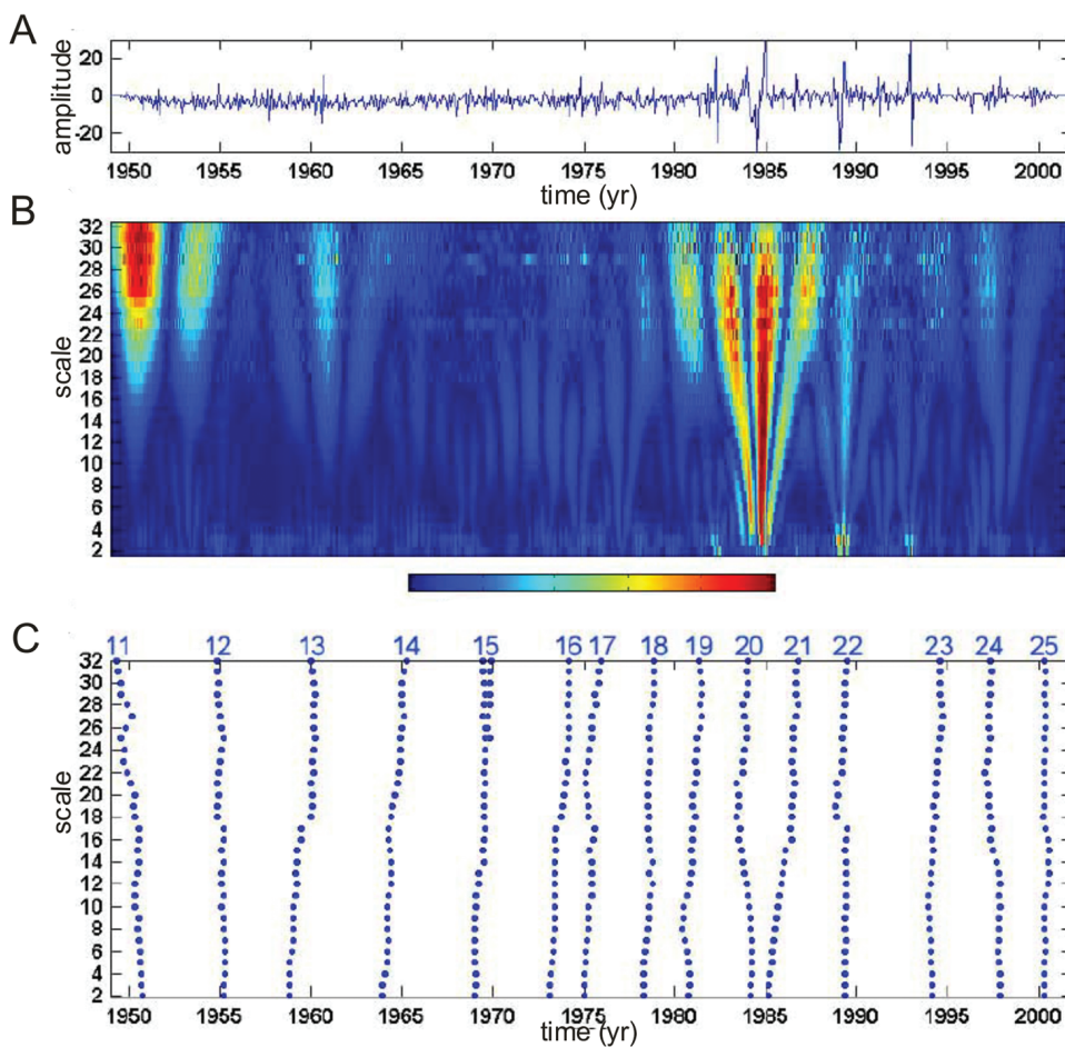
Figure 9 – In A, the secular variation of the Y component of the Vassouras observatory, from 1948 to 2001, in B the continuous wavelet transform and in C the lines of maxima coefficients of the wavelet transform.
