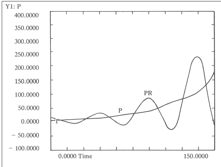
Figura 3: P and PR
