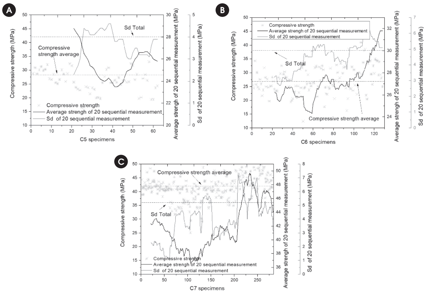
Figure 6 Compressive strength results of C5, C6 and C7 mixtures
