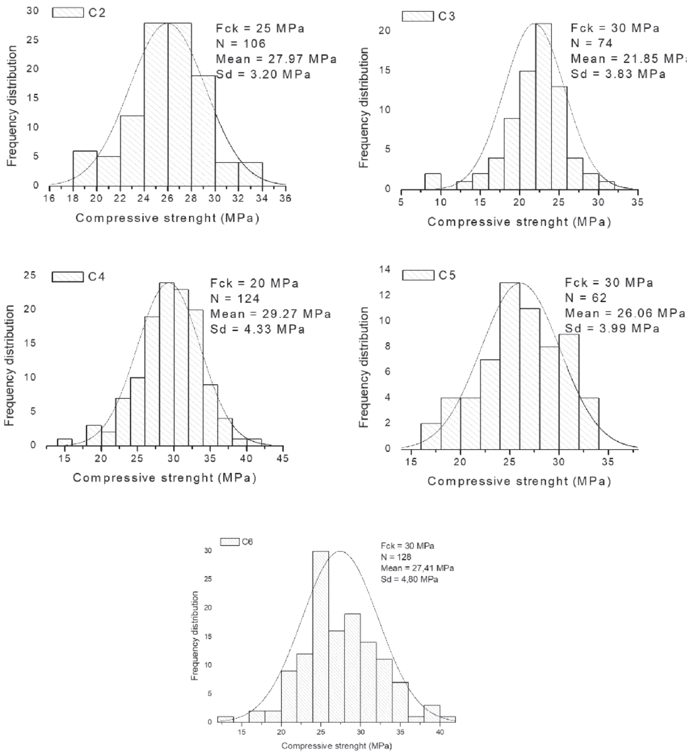
Figure 4 Normal distribution of the compressive strength values of the concretes side-mixed
