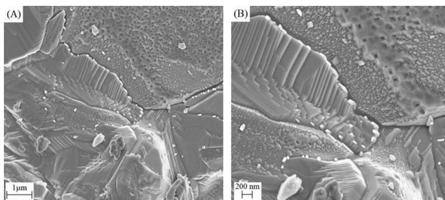
Figure 5: Scanning electron microscopy of CuFe 2 O 4 sample obtained at pH 5 (1000 °C / 2 h) conditions. (A) 1 µm and (B) 200 nm.
