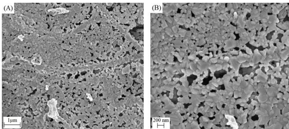
Figure 6: Scanning electron microscopy of CuFe 2 O 4 sample obtained at pH 7 sample (1) conditions (800 °C / 7 h). (A) 1 μm and (B) 200 nm.
