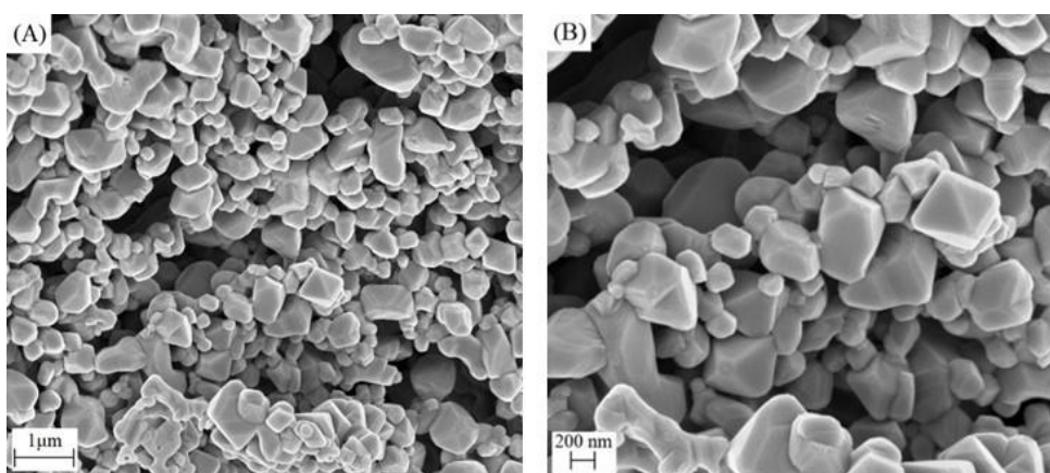
Figure 7: Scanning electron microscopy of CuFe 2 O 4 sample obtained at pH 7 sample (2) conditions (800 °C / 7 h). (A) 1 μm and (B) 200 nm.
