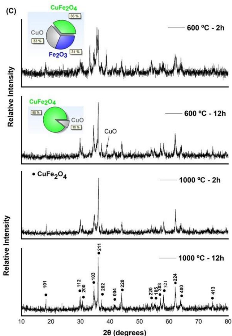
Figure 2: Copper Ferrite Diffractograms (A) pH 5, (B) pH 7 e (C) pH 9.
