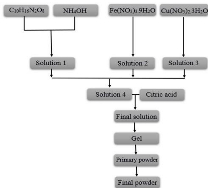
Figure 1: Proposed methodological route for \text{CuFe}_2\text{O}_4 synthesis based on the EDTA-Citrate complexation method.
