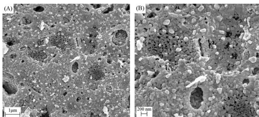
Figure 3: Scanning electron microscopy of CuFe 2 O 4 sample obtained at pH 5 (600 °C / 2 h) conditions. (A) 1 µm and (B) 200 nm.
