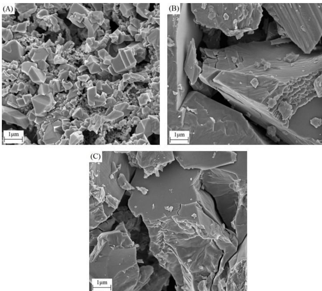
Figure 10: Scanning electron microscopy of CuFe 2 O 4 sample obtained at pH 9 conditions - 1 µm (A) 600 °C / 2 h, (B) 1000 °C / 2 h and (C) 1000 °C / 12 h.
