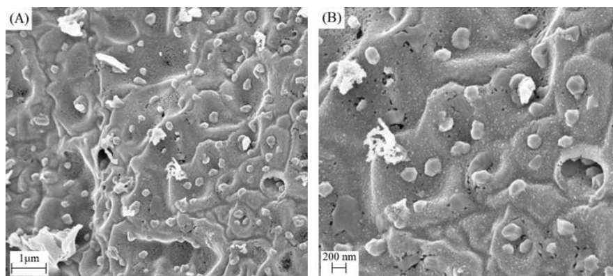
Figure 4: Scanning electron microscopy of CuFe 2 O 4 sample obtained at pH 5 (600 °C / 12 h) conditions. (A) 1 µm and (B) 200 nm.
