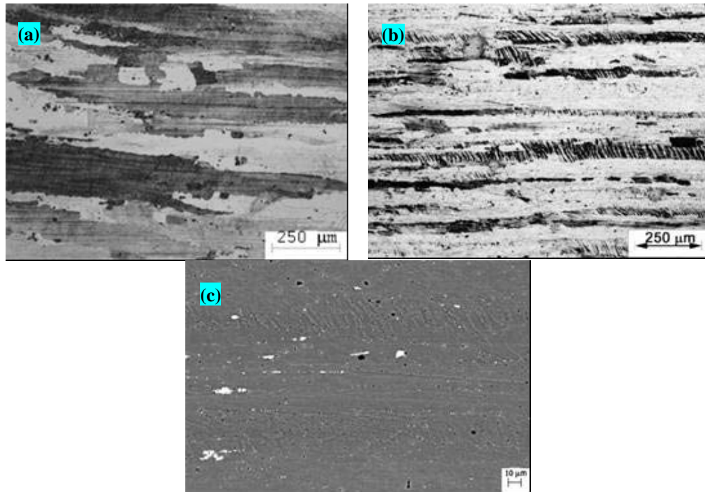
Figure 1: (a) Microstructure of 7050Al alloy in W condition. (b) and (c) Microstructures of 7050Al alloy after one pass of ECAP at Tamb, OM and SEM, respectively.
