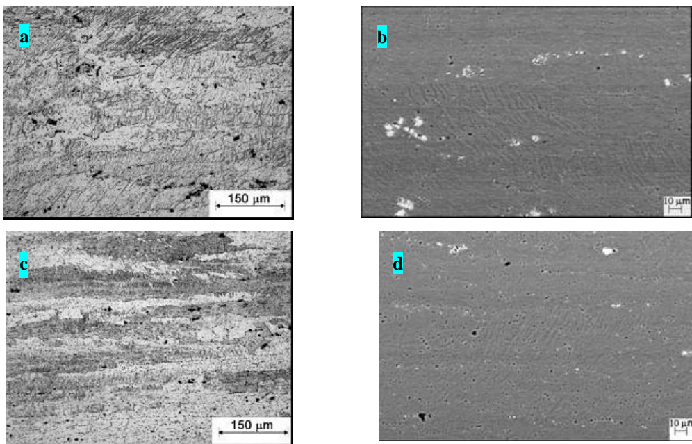
Figure 4: Microstructure of 7050Al alloy after ECAP at 150°C by route B C . (a) and (b) three passes; (c) and (d) six passes. (a), (c) OM; (b), (d) SEM.
