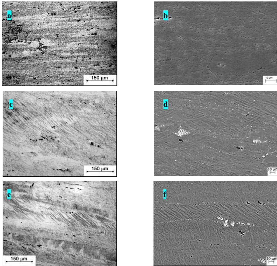
Figure 3: Microstructure of 7050Al alloy after ECAP at 150°C by route A. (a) and (b) one pass; (c) and (d) three passes; (e) and (f) six passes. (a), (c), (e) OM; (b), (d), (f) SEM.
