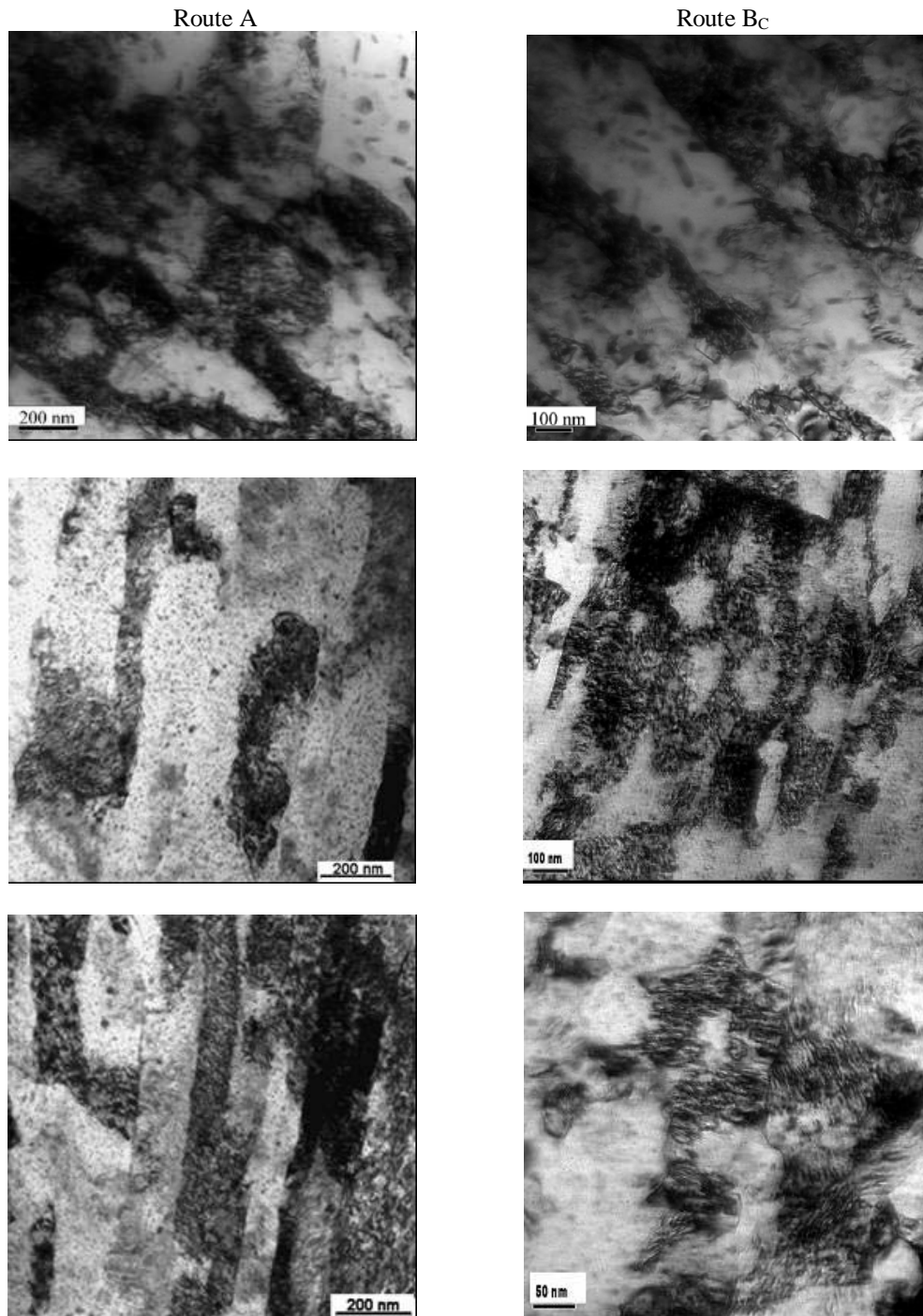
Figure 5: Microstructure by TEM of 7050Al alloy after ECAP at 150°C. (a) and (b) one pass; (c) and (d) three passes; (e) and (f) six passes.
