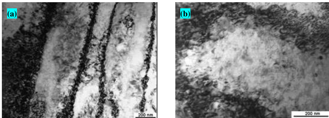
Figure 2: Bright field TEM images of 7050Al alloy after one pass of ECAP at Tamb.
