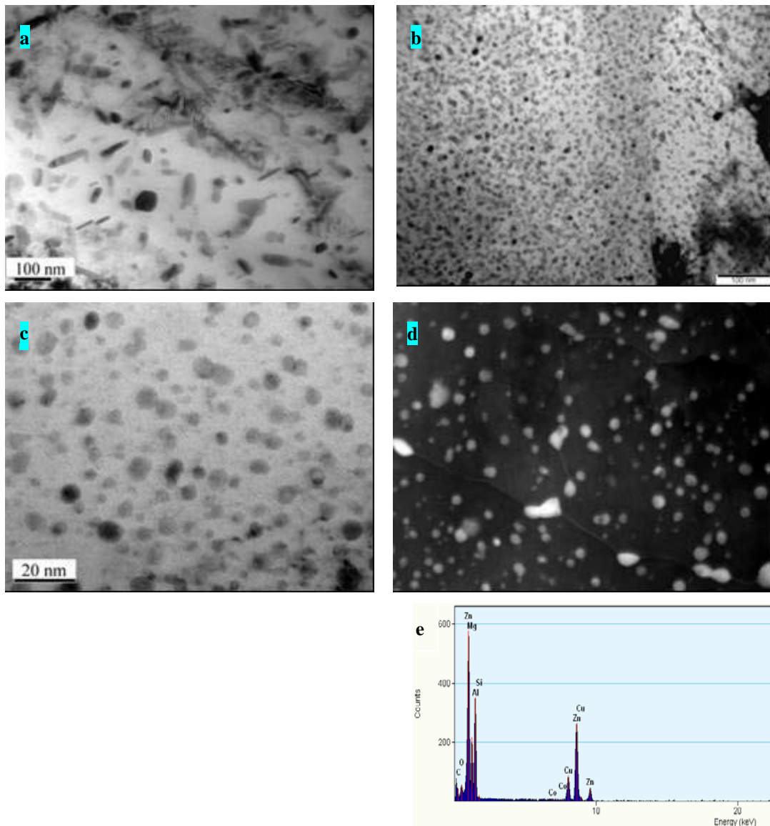
Figure 6: Microstructure by TEM of 7050Al alloy after ECAP at 150°C. (a) one pass; (b) three passes by route A (TEM); (c) six passes by route BC (BF – STEM); (d) six passes by route BC (HAADF image); (e) EDS spectrum of particle indicated in (d).
