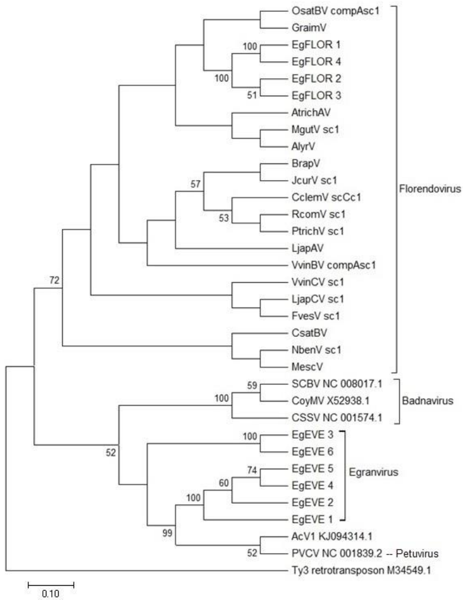
Figure S1 - Phylogenetic analysis of reverse transcriptase domain from EgEVE copies, compared to selected Caulimoviridae members. Ty3 retrotransposon was used as an external group.
