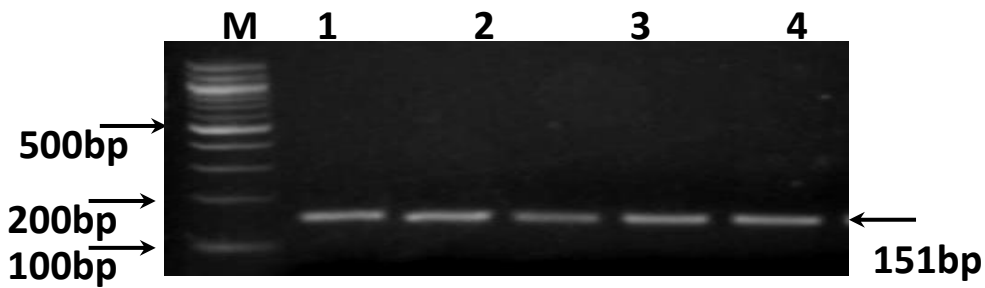
Figure S2 - A photograph of 2.5% agarose gel stained with ethidium bromide showing restriction digestion products. M represents 100 bp Molecular Weight Marker; Lane 1-4 Wild Type genotype; UD Undigested Product.
